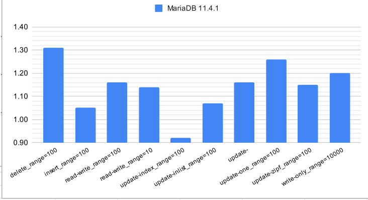
QPS relative to MySQL 8.0.36: writes, 4u,4t
