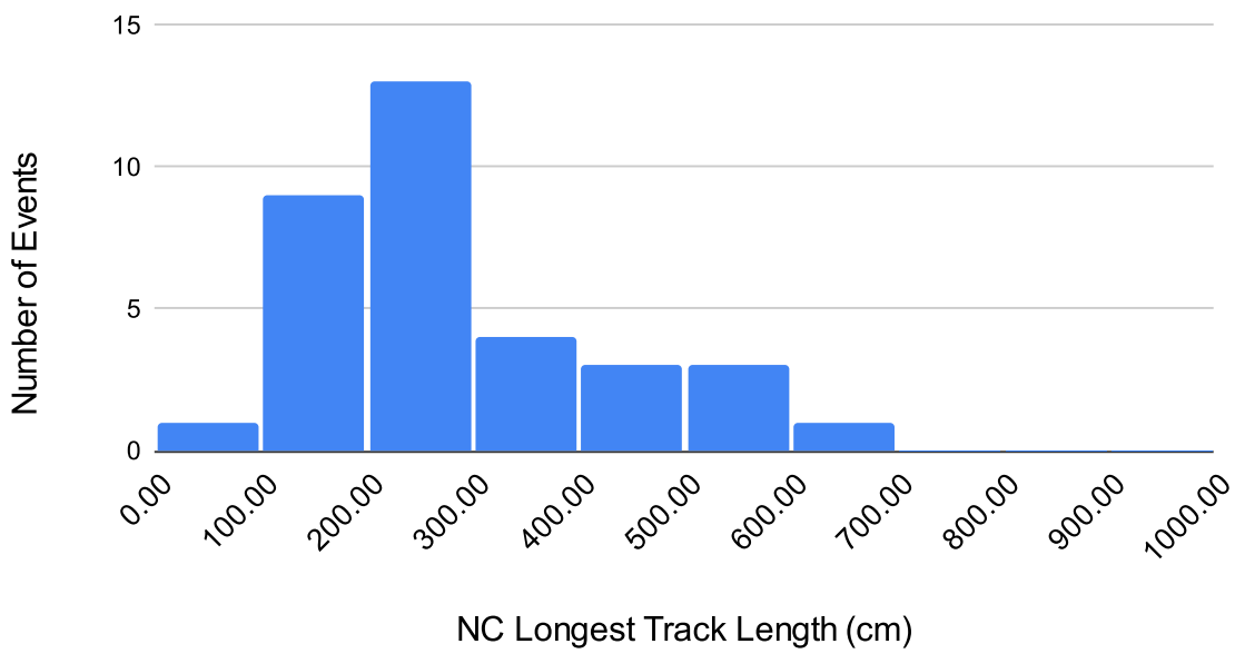
Histogram of Neutral Current Track Lengths
