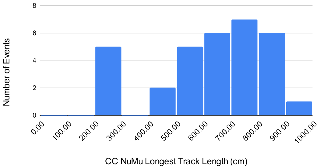
Histogram of Charged Current Track Lengths
