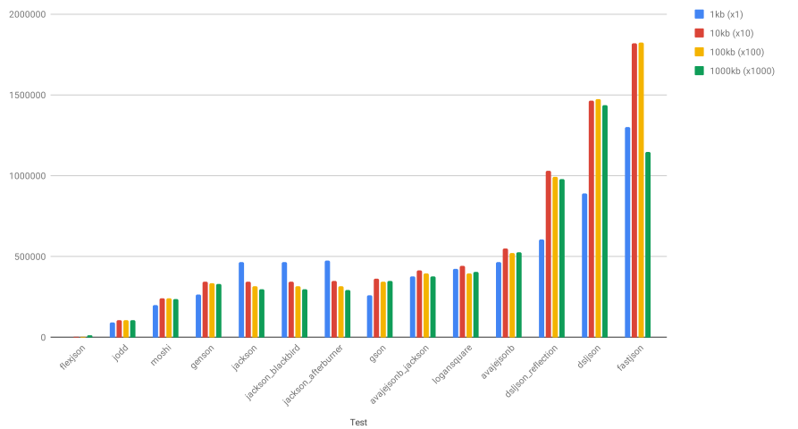
Serialization of various payload sizes - ops/s (higher is better)
