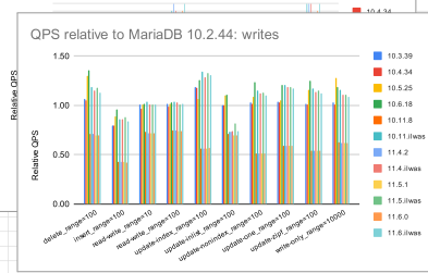
QPS relative to MariaDB 10.2.44: range queries, part 2
