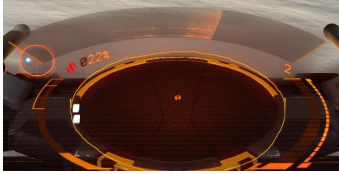
Outcrop
