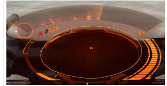
Metallic Meteorite
