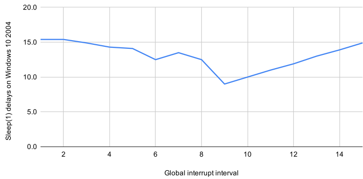
Sleep(1) delays on Windows 10 2004 vs. Global interrupt interval
