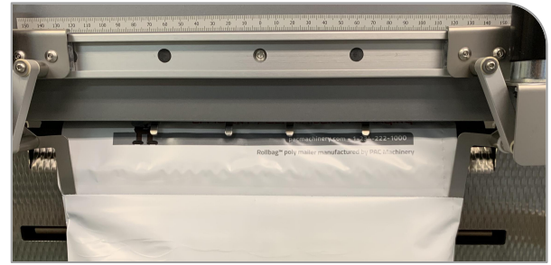
Seal flattener fingers go into the bag and stretch the top tight during sealing, to create a straight and clean final seal appearance
