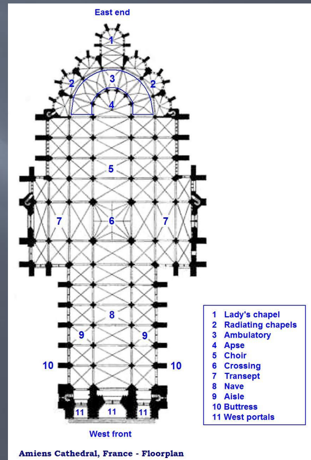
Amiens Cathedral, France - Floorplan
