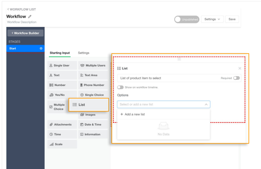
'List' on Workflow template builder in admin panel
