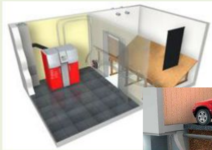
Figure 15, Selected internal and external pellet storage options
