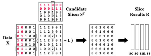
Figure 2: Example Vectorized Slice Evaluation (The matrix X has two red/black features, with 2/3 distinct values. The matrix multiplication (X \odot S^T) evaluates predicates by multiplying the one-hot vectors and counting matching predicates. By checking for (X \odot S^T) = L , we get rows that match all L slice predicates).
