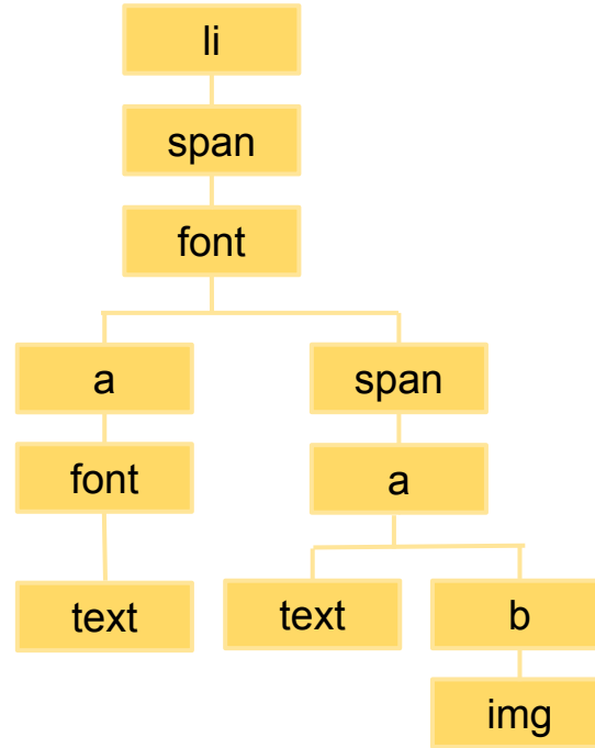
DOM Tree
