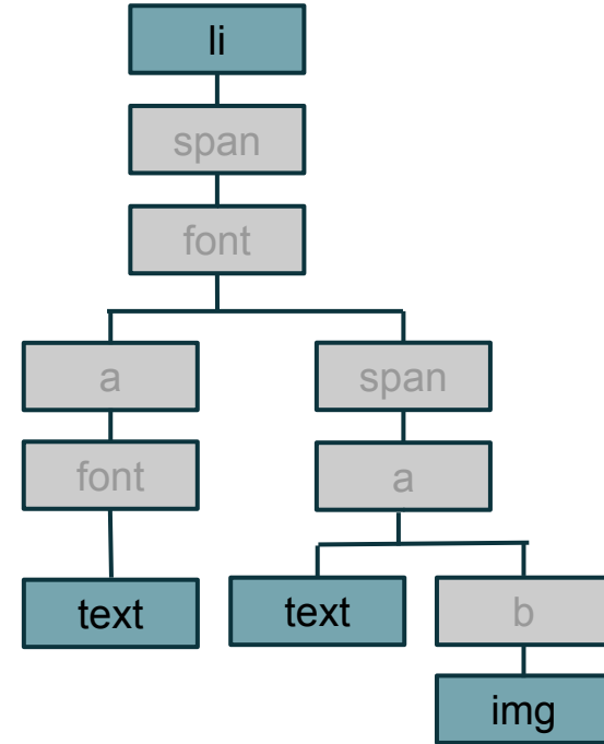
Culled inline box tree
