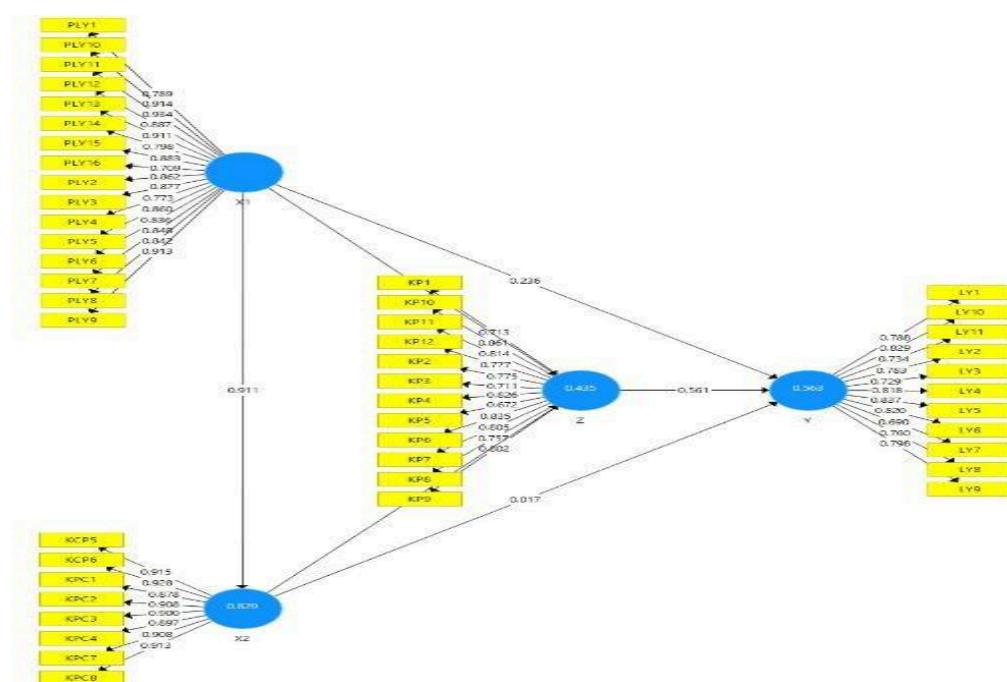
Figure 1. Path Coefficients
