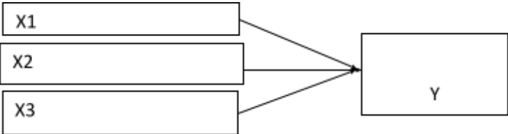
Figure 1. Conceptual Framework
