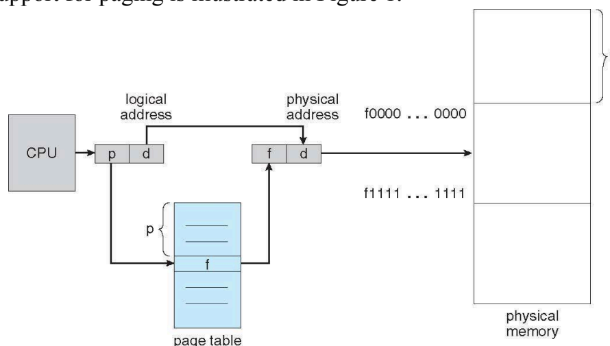
Figure 1: Paging hardware
