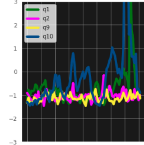
QuantilesS_RR_10M z_score(adj_ma_12m) Average normalized score trend for each quantile over time
