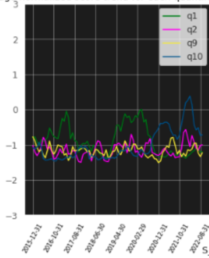
QuantilesS_RR_10M z_score(adj_ma_60m) Average normalized score trend for each quantile over time
