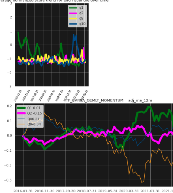
QuantilesTP_BARRA_GEMLT_MOMENTUM z_score(adj_ma_12m) Average normalized score trend for each quantile over time
