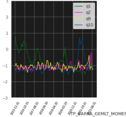
QuantilesTP_BARRA_GEMLT_MOMENTUM z_score(adj_ma_12m) Average normalized score trend for each quantile over time
