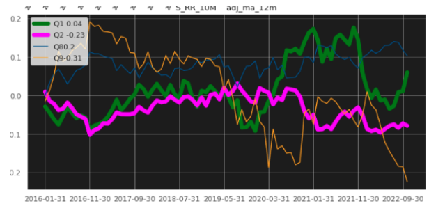
QuantilesS_RR_10M z_score(adj_ma_12m) Average normalized score trend for each quantile over time
