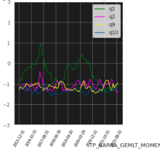
QuantilesTP_BARRA_GEMLT_MOMENTUM z_score(adj_ma_60m) Average normalized score trend for each quantile over time
