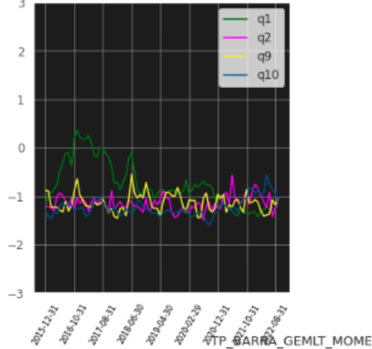
QuantilesTP_BARRA_GEMLT_MOMENTUM z_score(adj_ma_24m) Average normalized score trend for each quantile over time
