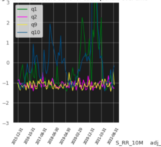
QuantilesS_RR_10M z_score(adj_ma_1m) Average normalized score trend for each quantile over time
