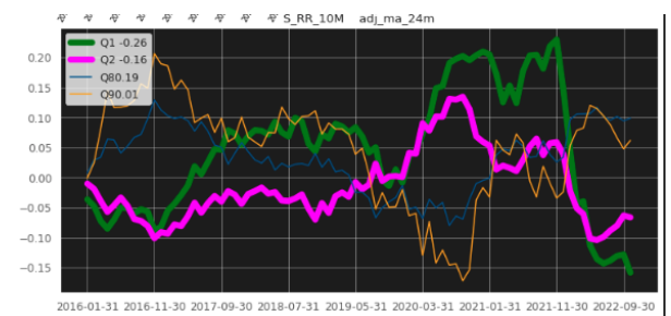
QuantilesS_RR_10M z_score(adj_ma_24m) Average normalized score trend for each quantile over time
