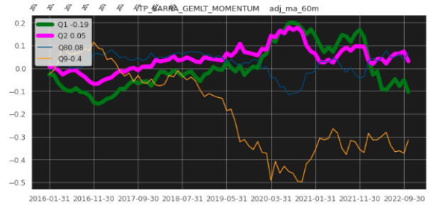
QuantilesTP_BARRA_GEMLT_MOMENTUM z_score(adj_ma_60m) Average normalized score trend for each quantile over time
