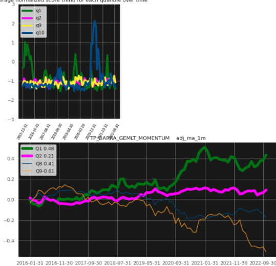
QuantilesTP_BARRA_GEMLT_MOMENTUM z_score(adj_ma_1m) Average normalized score trend for each quantile over time
