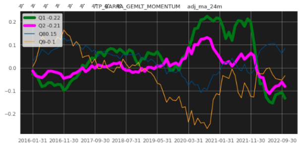
QuantilesTP_BARRA_GEMLT_MOMENTUM z_score(adj_ma_24m) Average normalized score trend for each quantile over time
