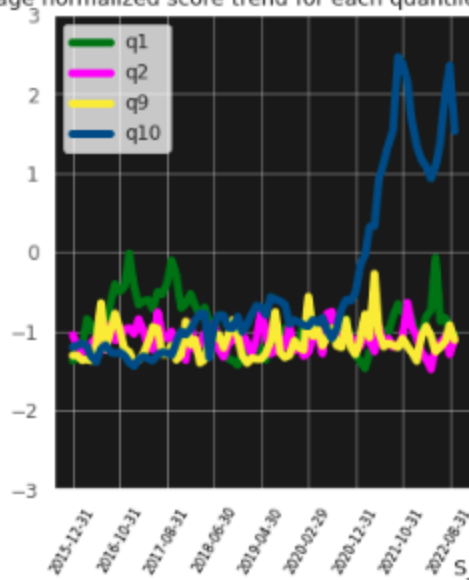
QuantilesS_RR_10M z_score(adj_ma_24m) Average normalized score trend for each quantile over time
