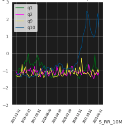
QuantilesS_RR_10M z_score(adj_ma_24m) Average normalized score trend for each quantile over time
