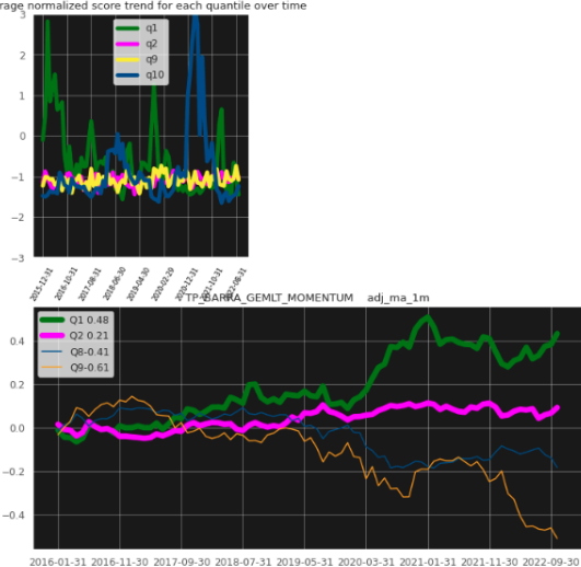
q1 max index 2016-02-29 max value 2.82 q10 max index 2021-03-31 max value 3.15 QuantilesTP_BARRA_GEMLT_MOMENTUM z_score(adj_ma_1m) Average normalized score trend for each quantile over time
