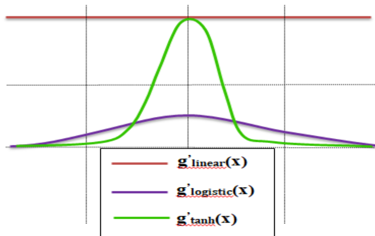
Fig – 4.2 Types of activation functions over graph
