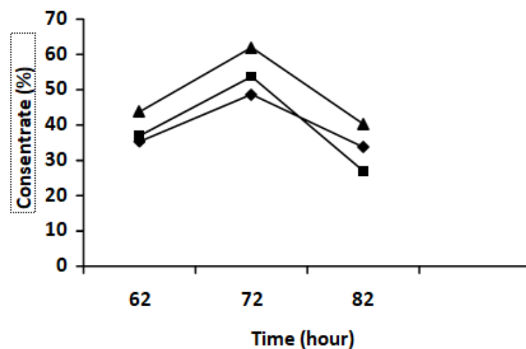
Picture 1. Curve of the effect of fermentation time on concentration Bioethanol ( ) Yeast 0,5g, ( ) Yeast 1g, ( ) Yeast 1,5 g
