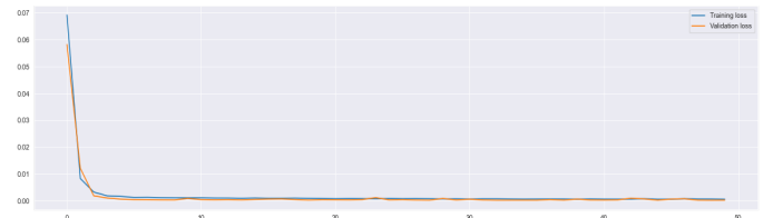
Figure 6: AR-LSTM: Training and validation loss with Twitter Data
