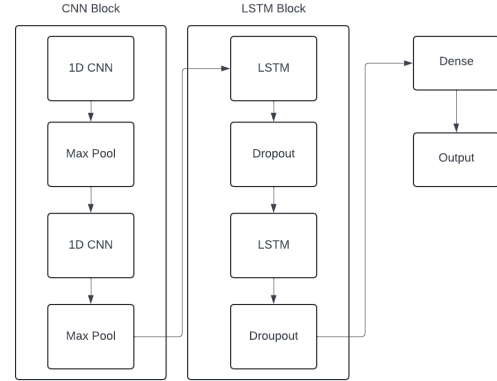
Figure 2: CNN-LSTM structure diagram
