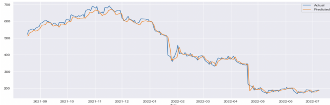
Figure 8: CNN+LSTM: Testing Prediction without Twitter Data
