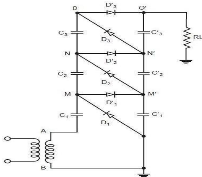
Figure: 3.3 multistage single phase cascade circuit of the Cockroft-Walton type
