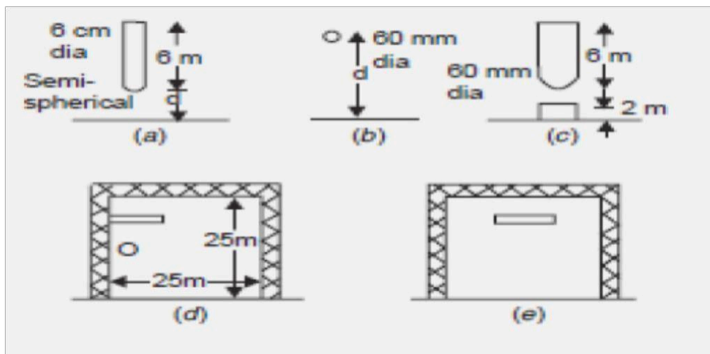
Figure: 1.9 Different gap geometries
