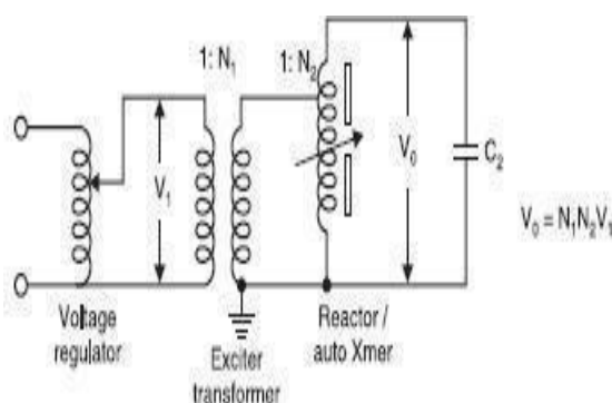
Figure: 3.17 Series-parallel resonant system
