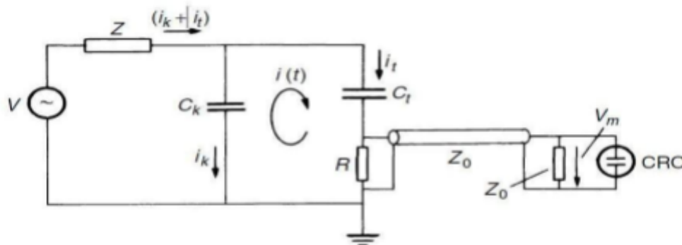
Figure: 5.11 Measurement of PD current low sensitivity circuit
