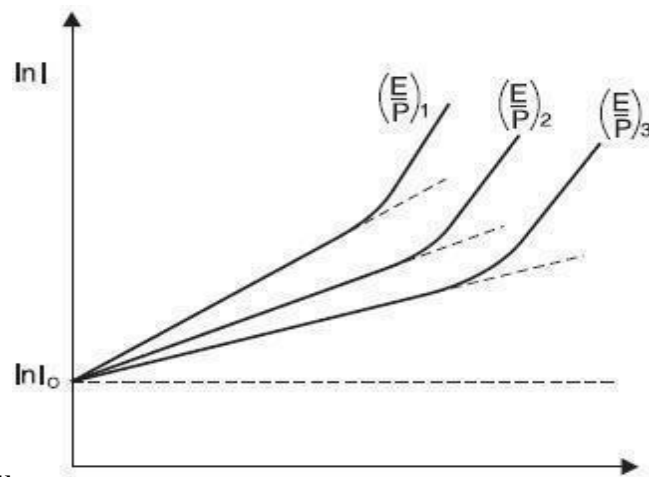
Figure. 2.5 variation of gap current with electrode spacing in uniform E
