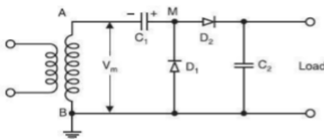
Figure: 3.2 Greinacher voltage doubler circuit
