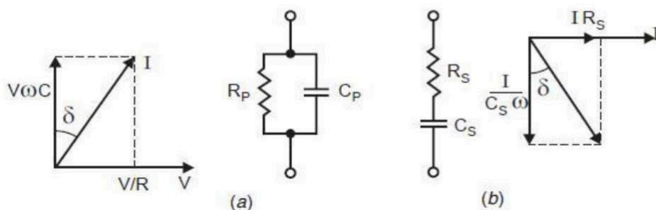
Figure: 5.8 Equivalent circuits for an insulating material
