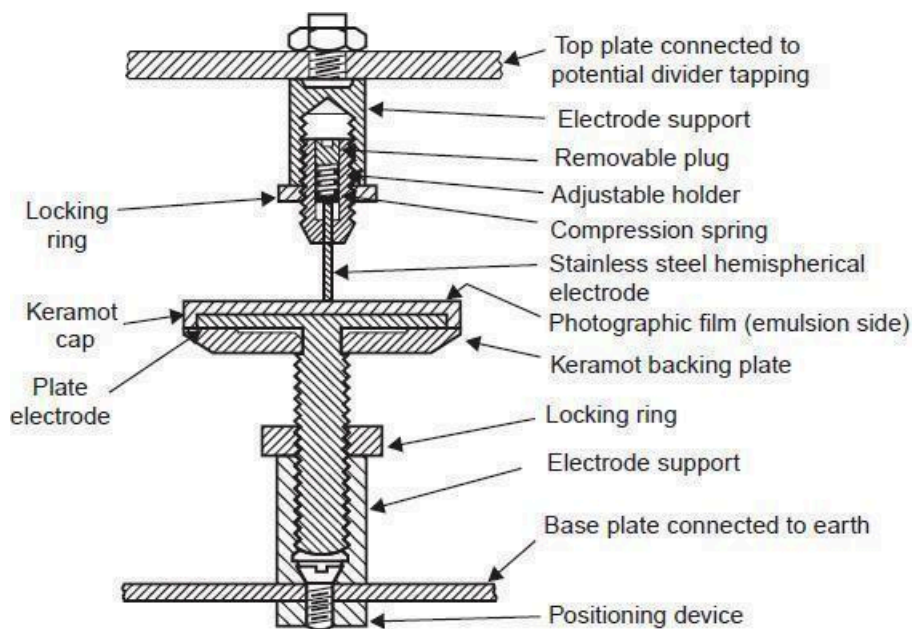
Figure: 4.16 Klydonograph
