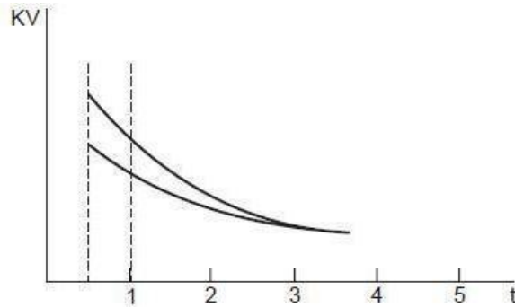
Figure: 5.1 Volt time curve of typical major insulation in transformer
