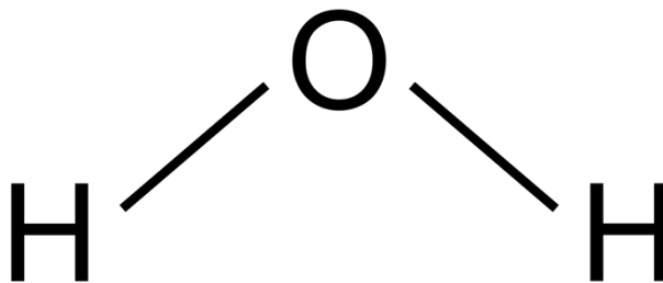
Figure 1. Chemical compound.
