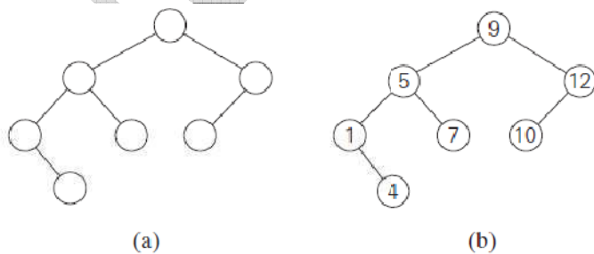
2 (a) Binary tree. (b) Binary search tree.
