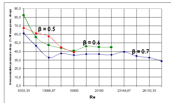
Gambar 14. Grafik prosentase irrecoverable pressure drop terhadap maximum pressure drop orifice plate 10 mm
