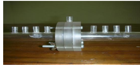
Gambar 3. Orifice plate flow meter
