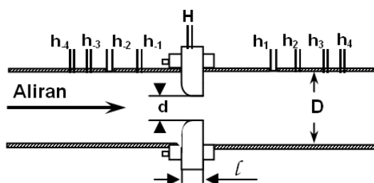
Gambar 2. Detail orifice plate
