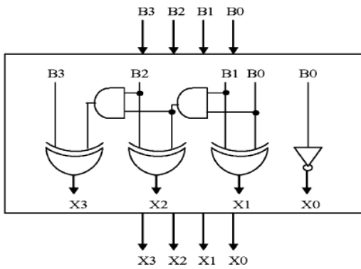
Figure 2: 4-Bit BEC
