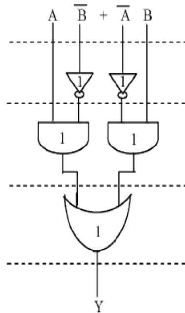
Figure 1: Delay and Area evaluation of an XOR gate. Table 1
