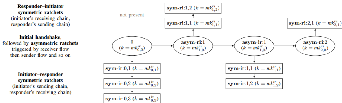
Figure 2. An example of an execution. Multiple stages of trees are formed. The content of each node is the stage name and the session key is derived during the stage.
