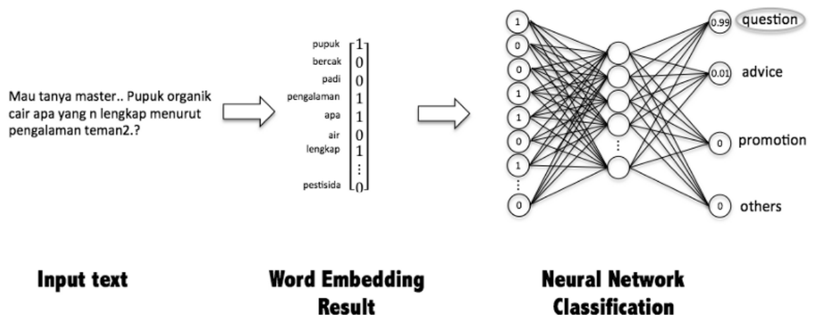
Figure 6. Process for intent classification using Neural Network
