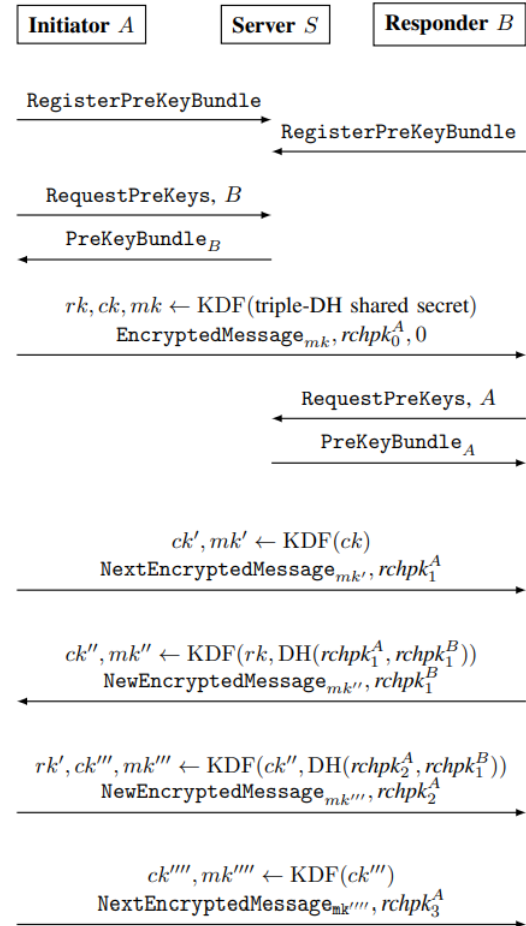
Figure 3. Message flow of an example execution between two clients A and B via a server S. Notation and some operations have been simplified for clarity compared to later use.
