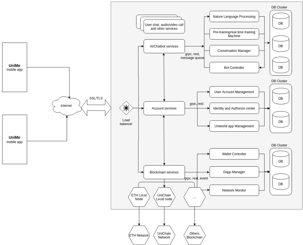
Figure 1. UniMe application high level architecture illustrated
