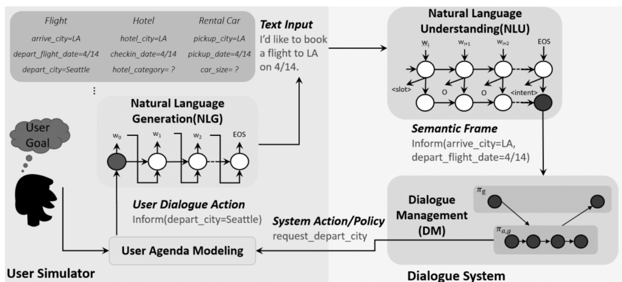
Figure 5. Chatbot based on Deep Learning
