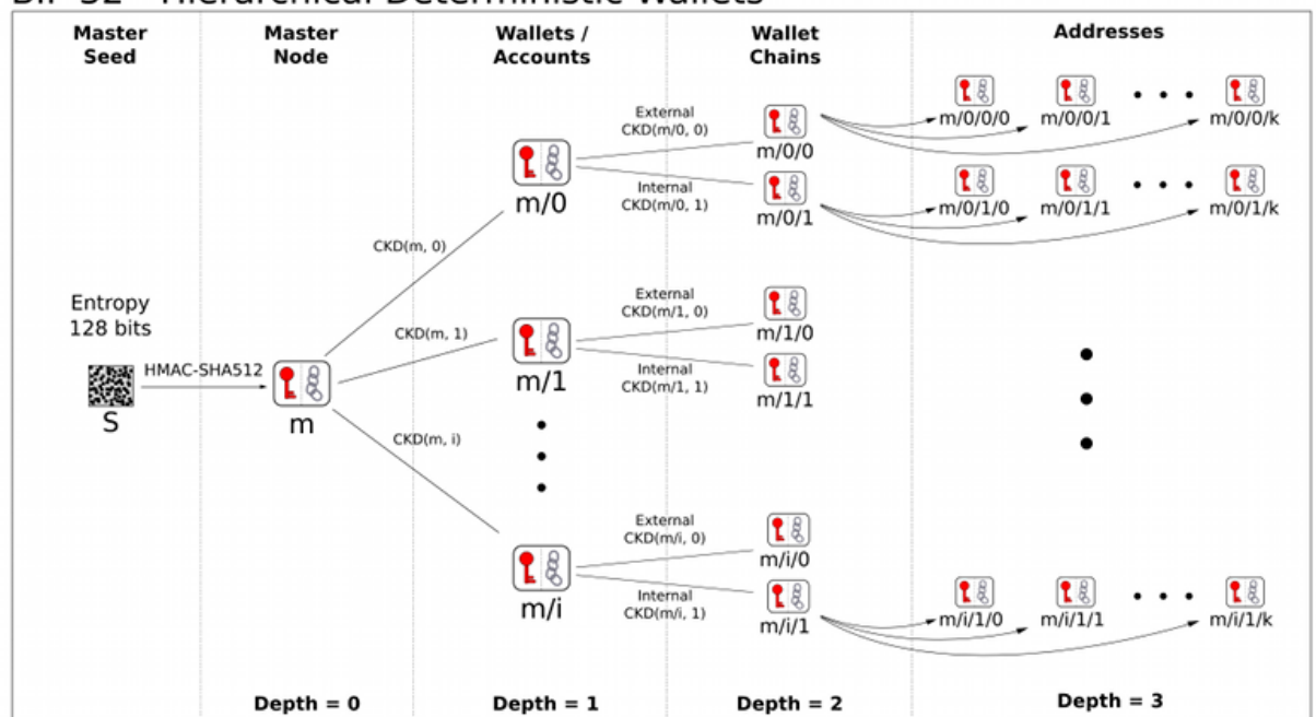
Figure 8. Key derivation from BIP32
