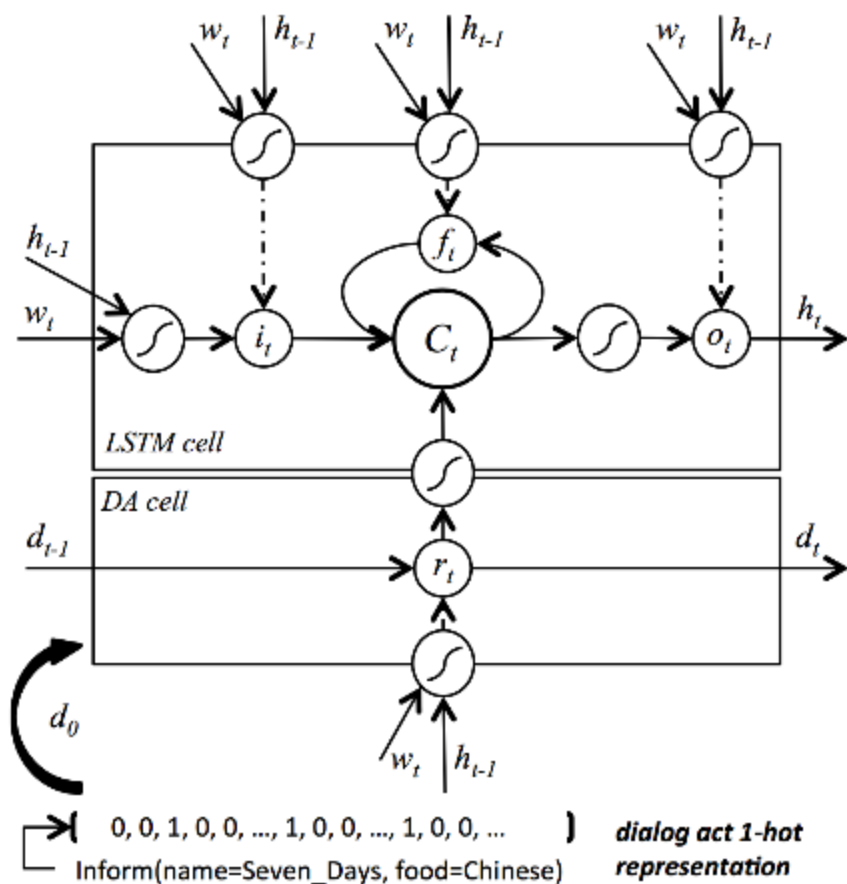
Figure 7. Semantic Controlled LSTM cell
