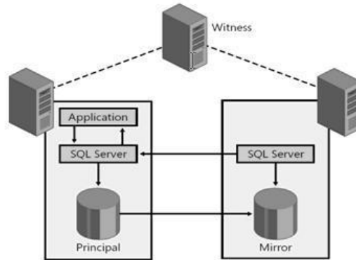
Gambar 1. Database Mirroring Therapy
