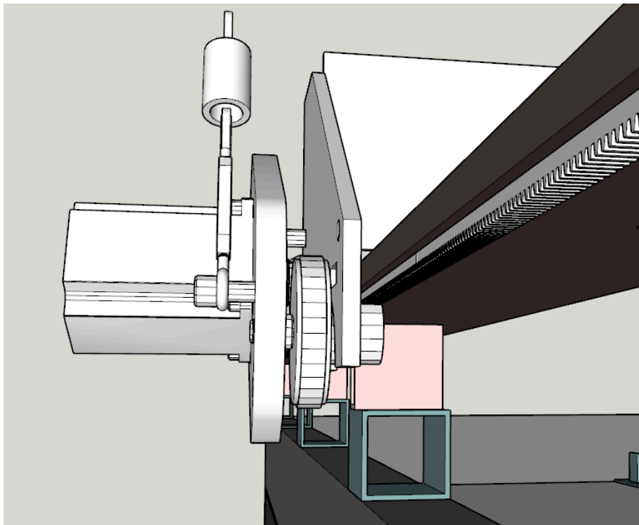
Gantry Drive and Side Plates
