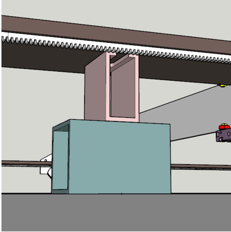
Gantry Drive and Side Plates
