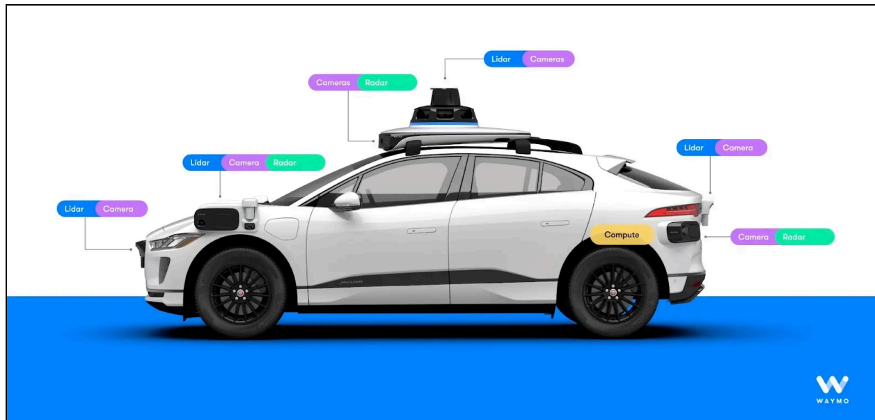
Figure 11. Indicates locations of LiDAR, radars, and cameras around the Waymo Jaguar I-PACE. [60]
