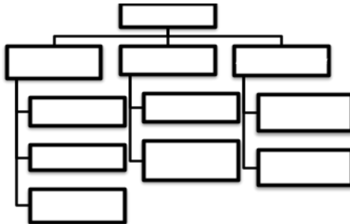
Gambar 1. Fraud Tree
