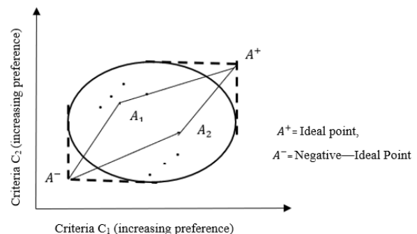
Figure 1 Basic concept of TOPSIS (Browallia New 12)
