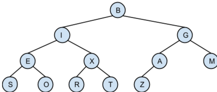
Heap Construction [Initial State]
