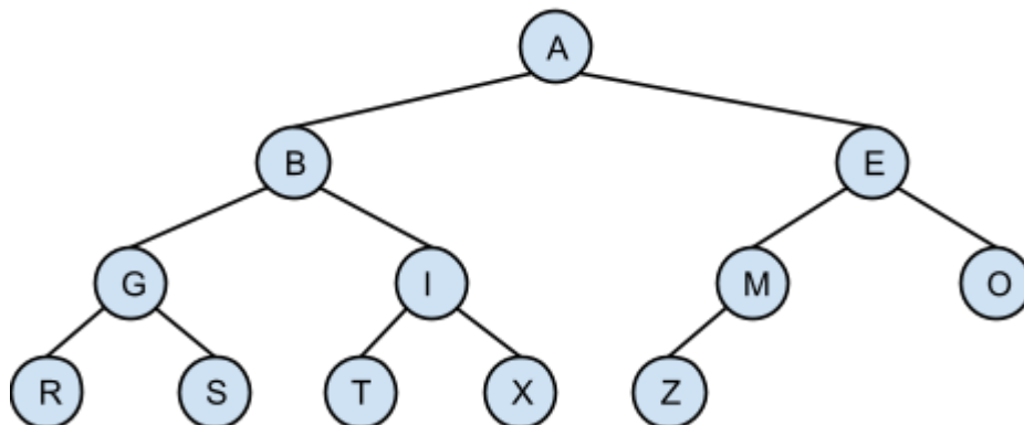
[Sorted State]
