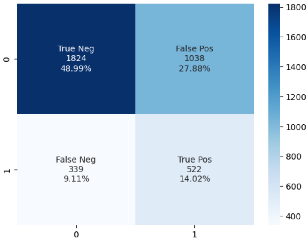
Figure 1. Heatmap of Logistic Regression Confusion Matrix
