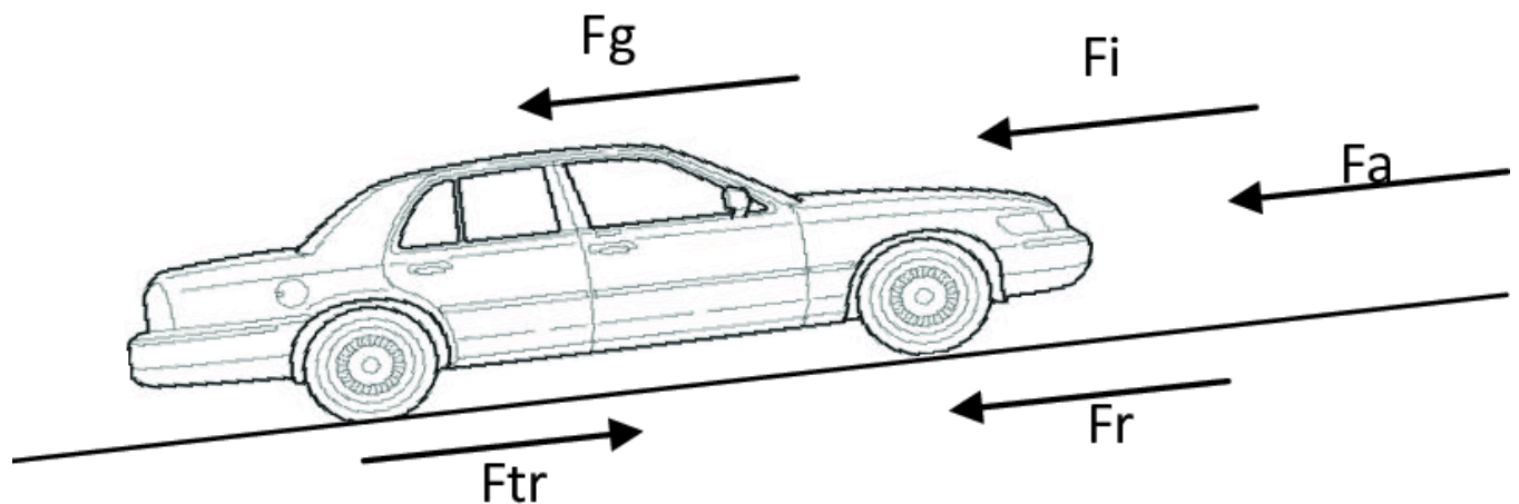
Figure 1 tractive forces free body diagram
