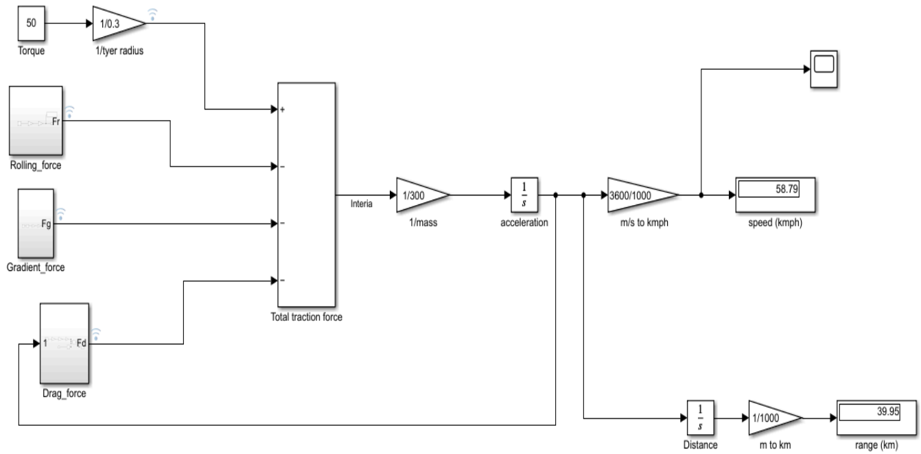
Figure 2 Simulink Model of Speed Torque Characteristic Model
