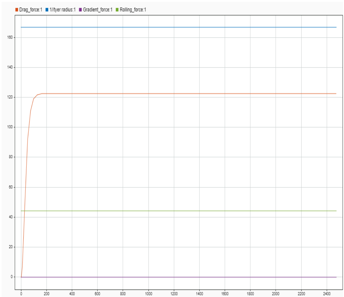
Figure 3 Force Asserted on Vehicle Vs Time Curve
