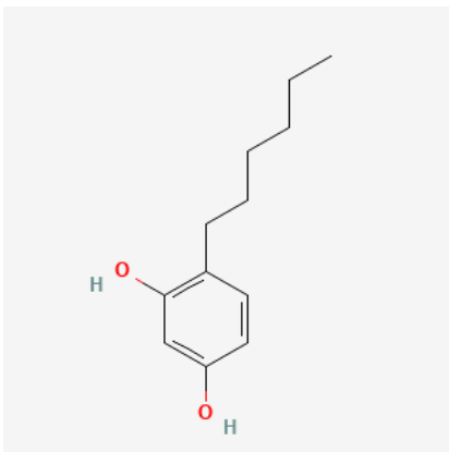
Figure 1. Structure of hexylresorcinol (Minimum resolution of 300 dpi), calibri, 10 pt
