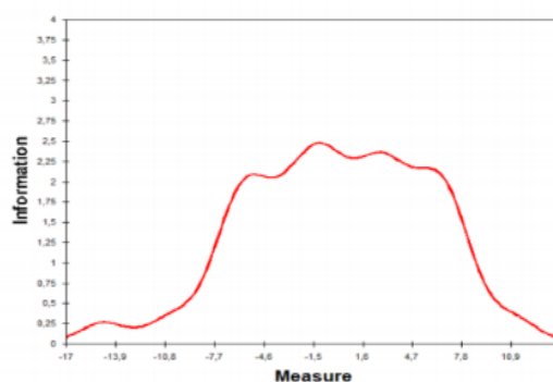
Figure 1. Test Information Function
