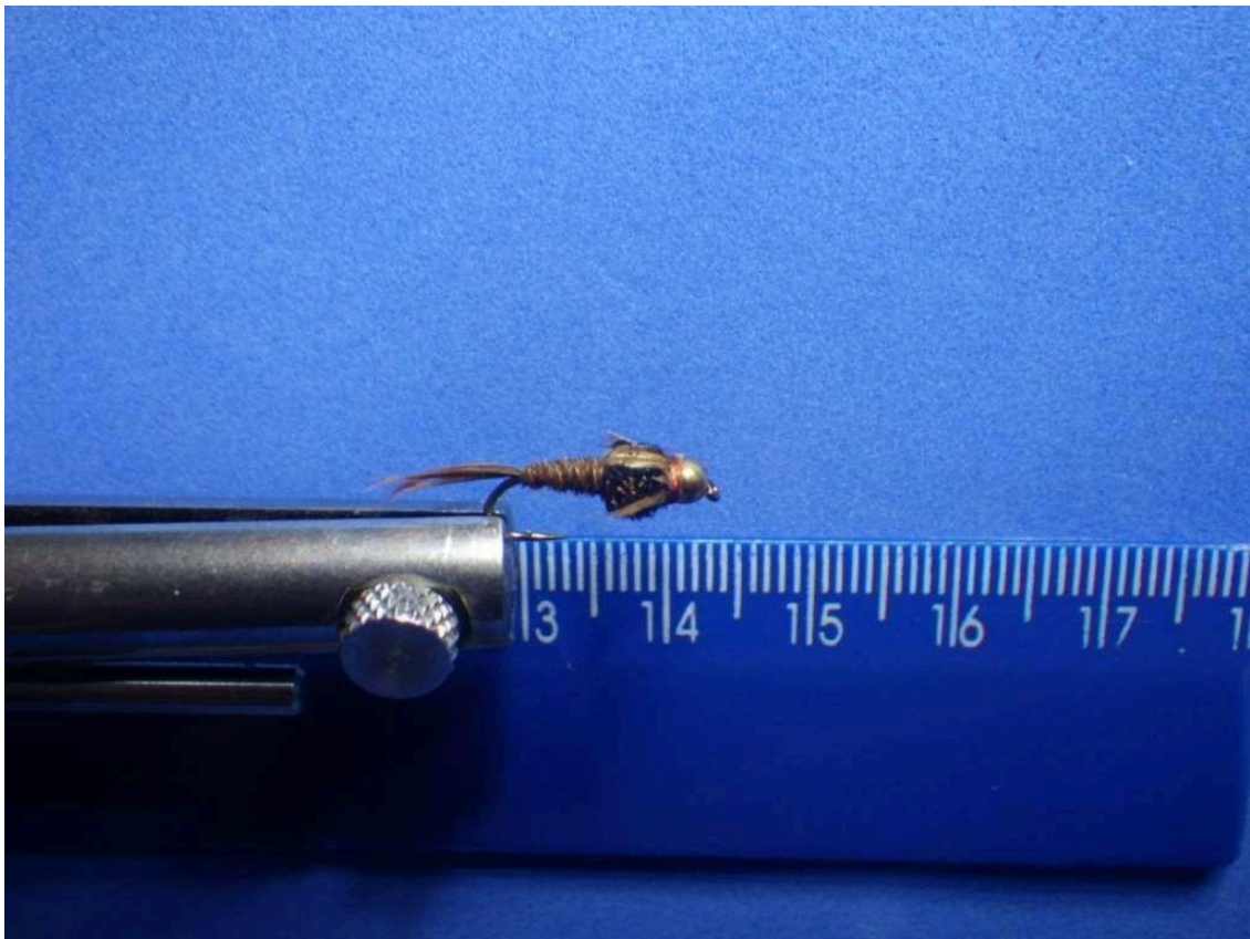
Bead Head Pheasant Tail Nymph (Anzol #14) Estoque: 06 moscas (Unidade: R$ 8,00)
