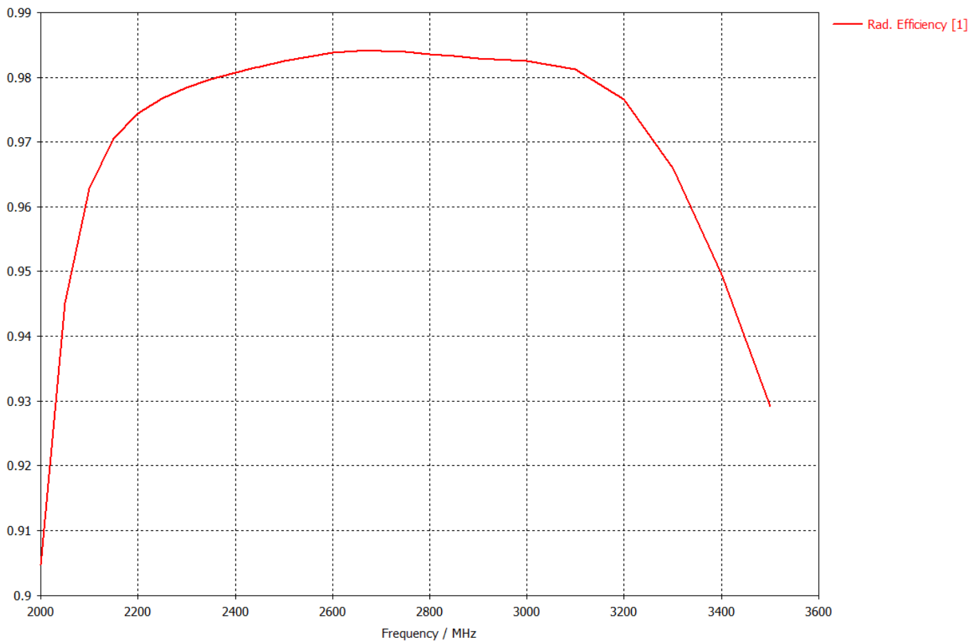
Radiation Efficiency [Magnitude]
