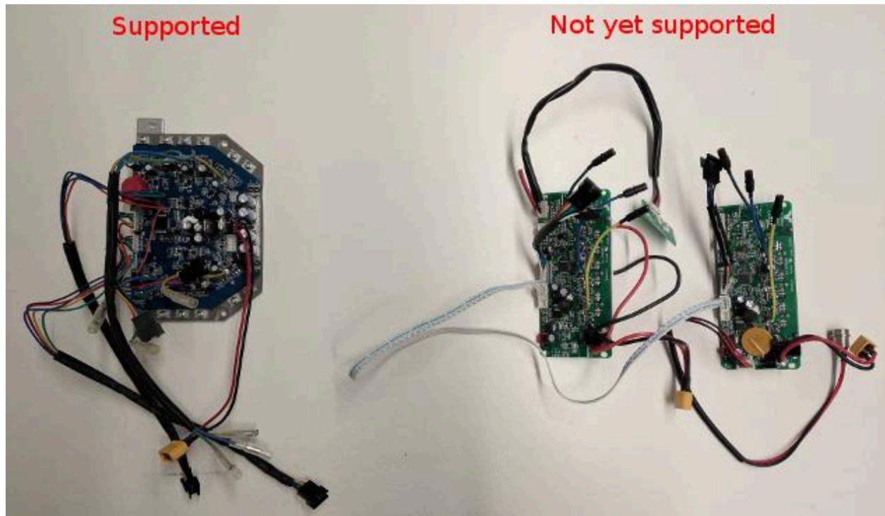
Supported single board on left, Unsupported dual motor controllers on right.
