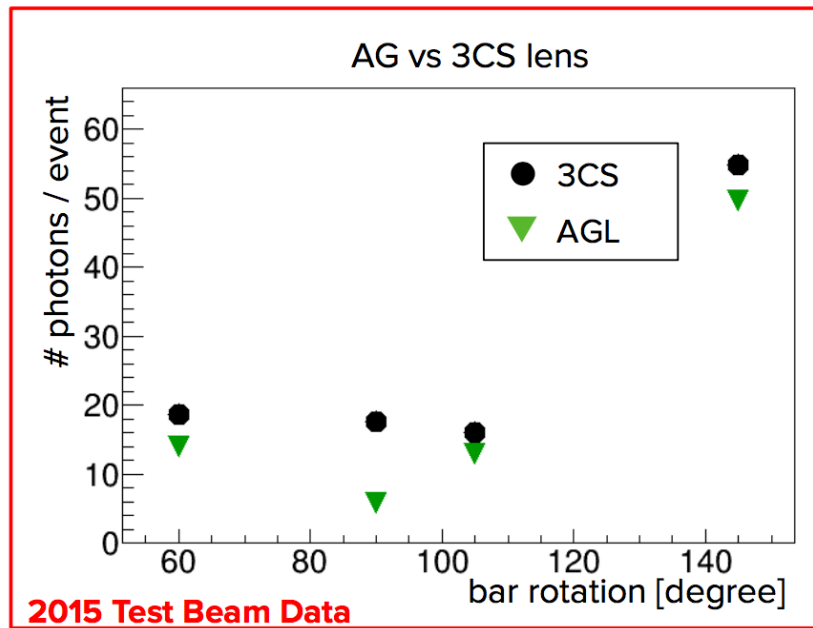
Figure 3.13. Photon yield as a function of beam polar angle for the 2015 CERN beam data. Green points: Setup with air-gap lens. Black points: Setup with 3-component lens.
