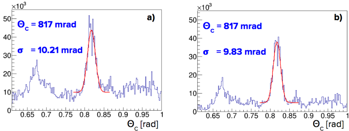
Figure 3.9. Reconstructed single-photon Cherenkov angle for simulated data using Geant4. 7 GeV/c protons are entering the setup with 3-component lens at a 125^\circ angle. Left: without time cut. Right: with 2-ns time cut (measured - expected).
