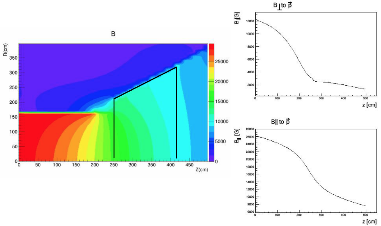
Figure 2.2.2.10: (left panel) Preliminary magnetic field map (in Gauss) in the (outgoing) ion side of the MEIC detector; the nominal region for the dual-radiator RICH detector is Z = [250,415] cm; (right panel) perpendicular and parallel components of the field to the momentum (for a track with polar angle of 25^\circ ).
