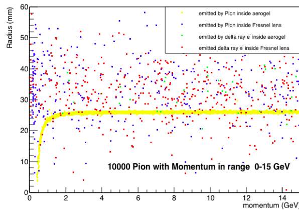
Figure 2.2.1.8. Radius vs Momentum. Yellow dots represent signal Cherenkov photons emitted by incident pions inside aerogel. Blue, green, and red dots represent background Cherenkov photons emitted by incident Pions inside Fresnel lens, by delta ray electrons inside aerogel, and by delta ray electrons inside Fresnel lens, respectively.
