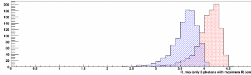
Figure 2.2.2.3. Histogram of mean radius of the spot of photons hits coming from CF 4 gas (for Pions in red and Kaons in blue); only 3 hits per spot with larger radius with respect to the track hit point have been selected.
