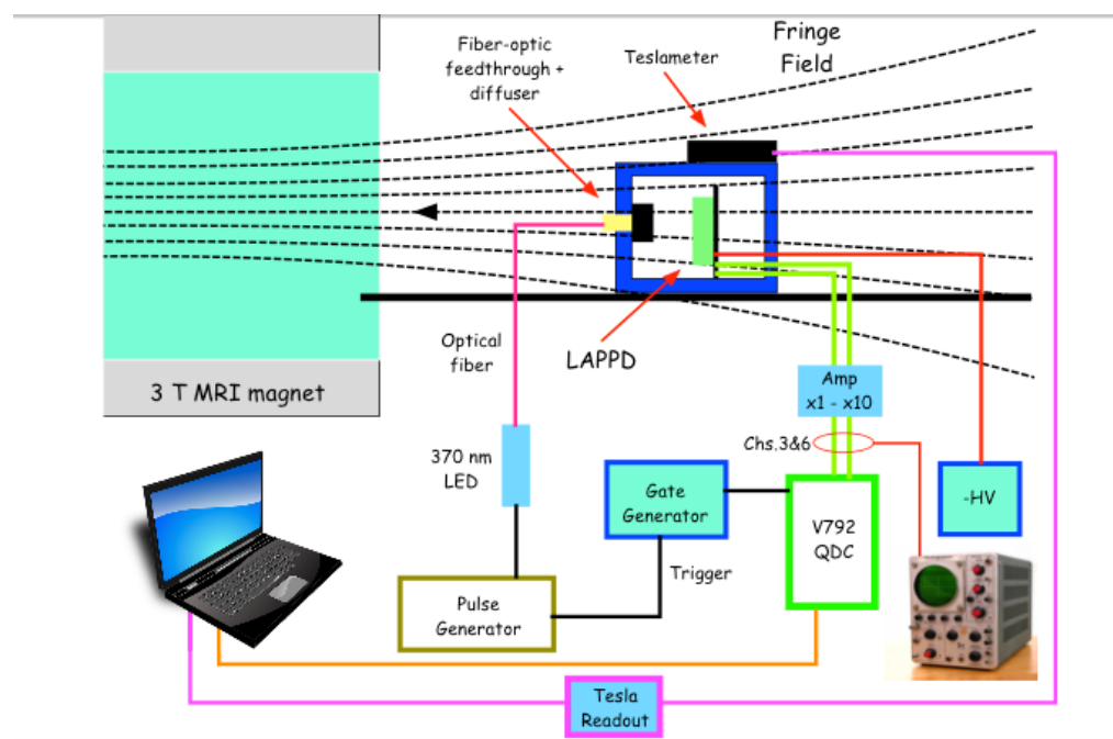
Figure 4.2.4. Schematic of the setup partially shown in the photo of Fig. 4.2.3.
