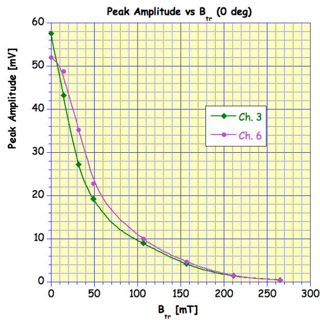
Figure 4.2.10. The loss in relative gain for the two channels as function of the transverse field.
