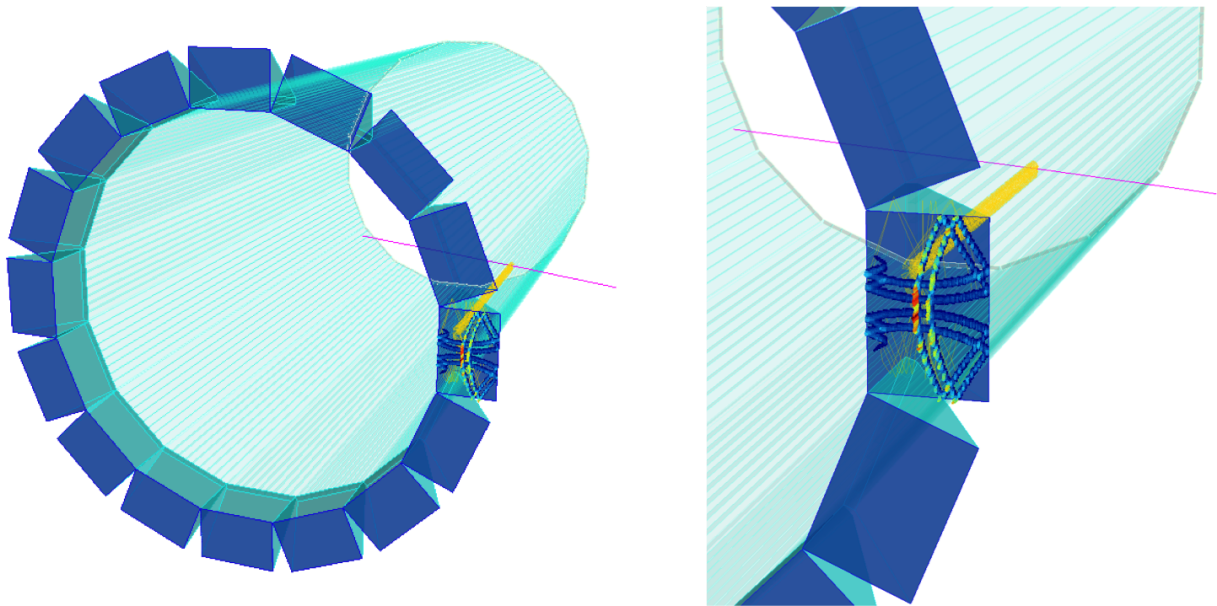
Figure 3.1. A Geant4 implementation of the tentative geometry of a lens-based, high-performance DIRC for the EIC with narrow bars and a solid fused silica prism. The simulated event shows the primary charged track in magenta, with Cherenkov photons in yellow.
