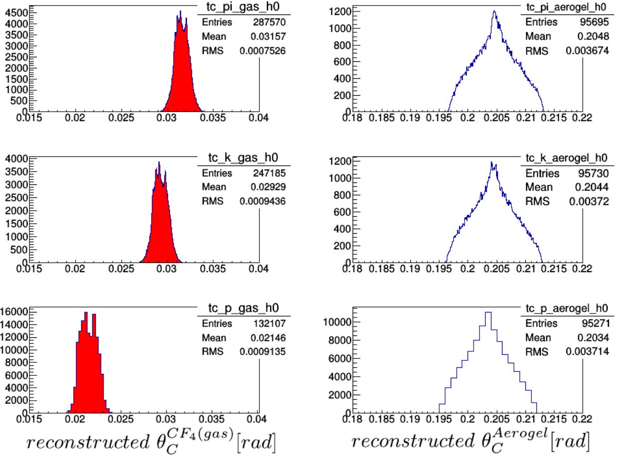
Figure 2.2.2.9: Distributions for the reconstructed gas (left panel) and aerogel (right panel) cherenkov angles (sample of 1000 tracks with momentum 40 GeV/c at polar angle of 25°) for \pi, K, p (from top to bottom).
