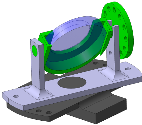
Figure 3.19. A CAT 3D image of the 3-layer lens holder designed for focal plane mapping.
