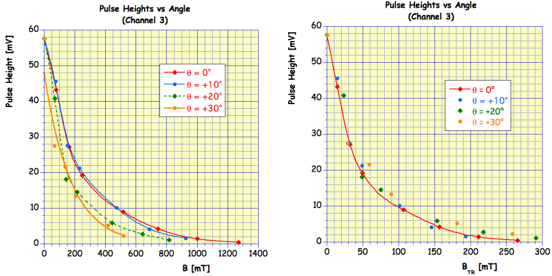
Figure 4.2.11. Pulse heights (relative gain) as a function of the B field (LH) and the transverse field (RH) for a variety of rotations on the platform plane. The data indicates that the transverse field is the correct parameter to use in analyzing the gain changes.
