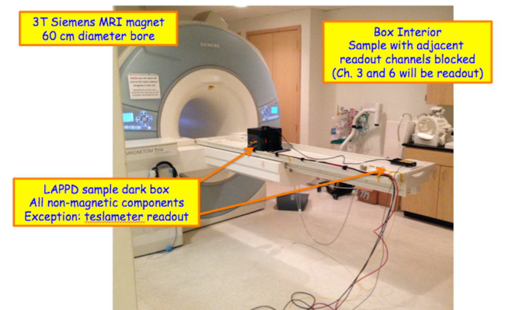
Figure 4.2.3. A photograph of the setup at the UVA MRI research facility (Dept. of Biomedical Engineering). The sample box was placed on platform that could be moved in small controlled steps (millimeters). The magnetic field strength was measured by a 3-axis teslameter [2]. All DAQ hardware and the PC laptop were placed outside the room as required for safe operation. Other than the teslameter readout box, all materials inside the room were non-magnetic.
