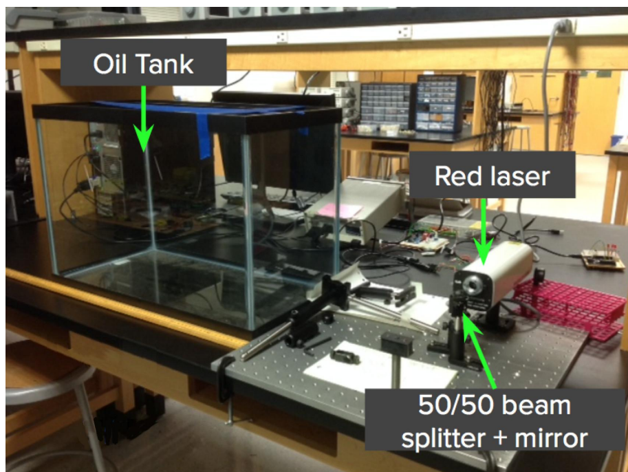
Figure 3.18. A photograph of the setup to map the lens focal plane built at ODU.
