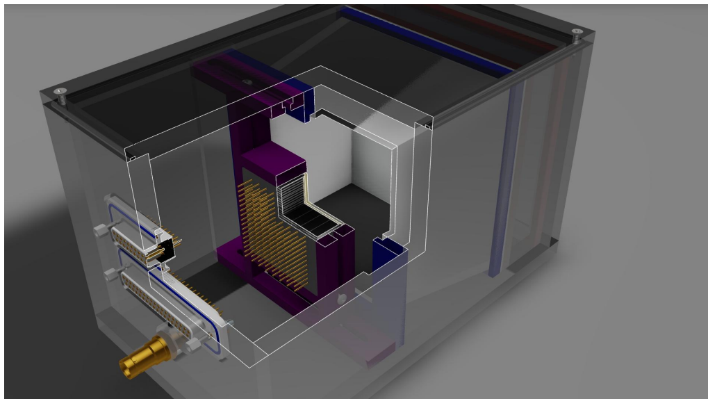
Figure 2.2.1.2. Prototype detector seen from the back. The cutout shows the multi-anode PMT.
