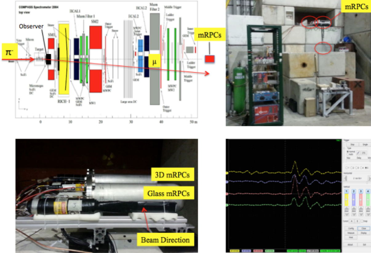
Figure 1.2.1.1: Top left diagram shows the COMPASS spectrometers and the location of the mRPCs is indicated with a red colored rectangle. The top right picture shows the test setup at the end of the COMPASS spectrometers. Bottom left shows two chambers for the glass mRPCs, 3D printed gas gap mRPCs, and scintillators for the trigger. Bottom right screen shot shows the signals from the glass mRPCs captured by the DRS4 waveform analyzer with a coincidence trigger.
