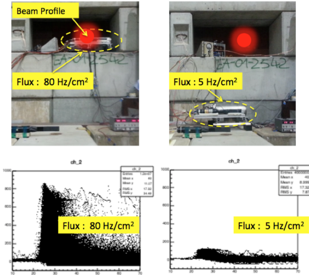
Figure 1.2.1.2. Top two pictures show the two locations for the test setup to vary the flux rate. The solid circles of red color in the pictures are estimated position of beam. The bottom two plots show the accumulated signals from mRPCs under the same gas mixture, 2% SF 6 , and high voltage, 22kV, except the location. The range of Y-axis on the plots is from -10mV to 1000mV, and the X-axis is time from 10 ns to 70 ns.
