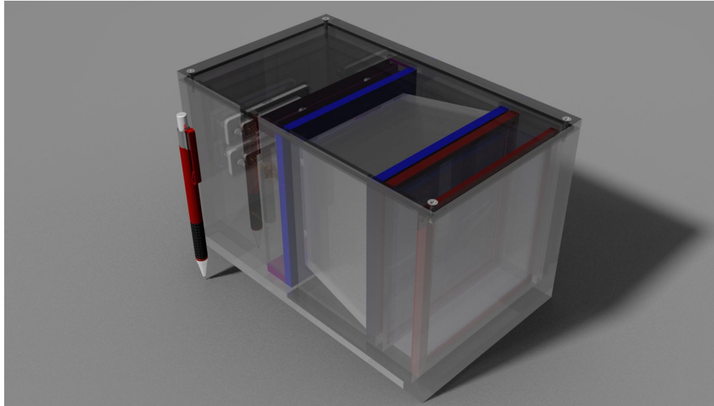
Figure 2.2.1.1. Prototype detector design seen from the aerogel side.
