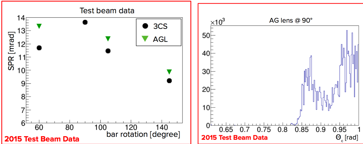
Figure 3.11. Left: Single-photon Cherenkov angle resolution as a function of beam polar angle for the 2015 CERN beam data. Green points: Setup with air-gap lens. Black points: Setup with 3-component lens. Right: Reconstructed single-photon Cherenkov angle for 90° polar angle and air-gap lens setup.
