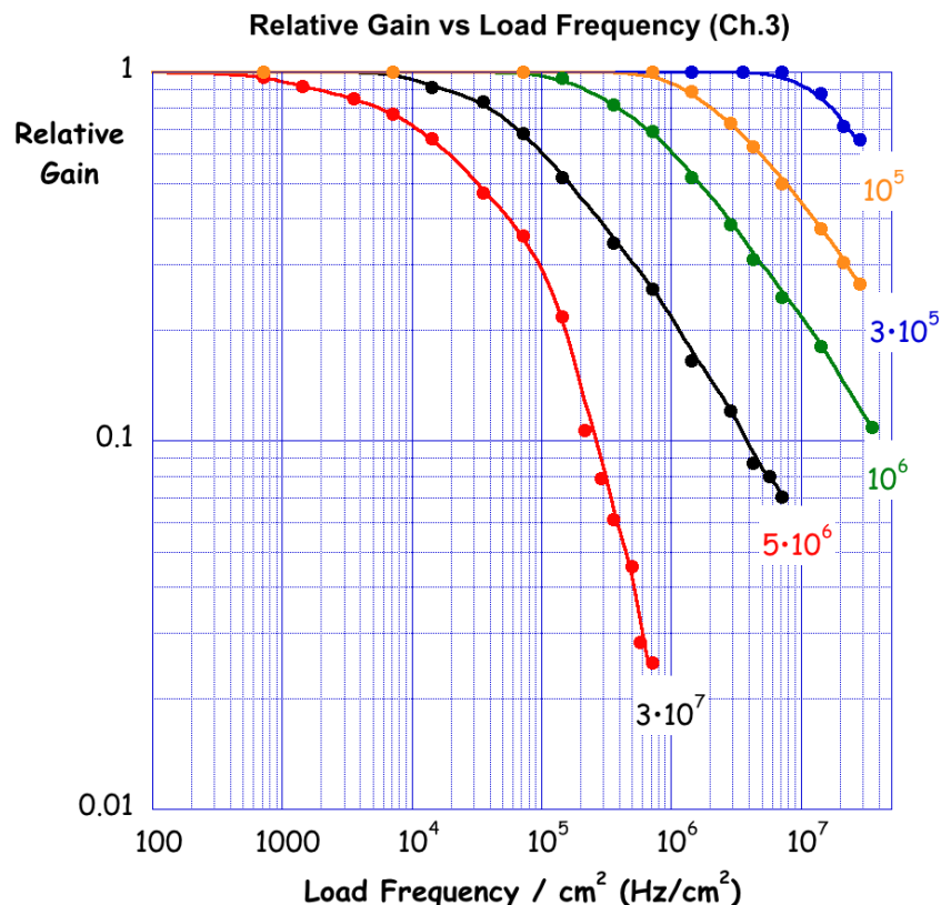
Figure 4.2.14. Results of an initial rate test of the LAPPD sample for one readout channel. The rates are normalized to 1 cm 2 . The pulsed load was tuned to produce a mean count of 0.5 photoelectrons per pulse.
