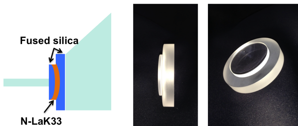
Figure 3.2. Schematic diagram and two photos of the prototype three-layer spherical lens.
