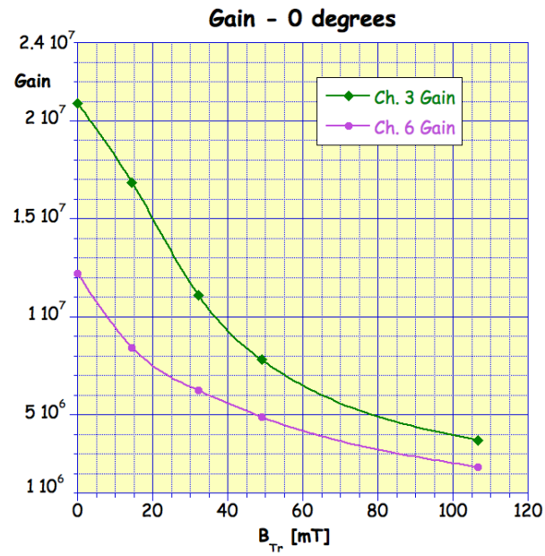
Figure 4.2.9. The loss in absolute gain as a function of the transverse field for the two monitored channels.
