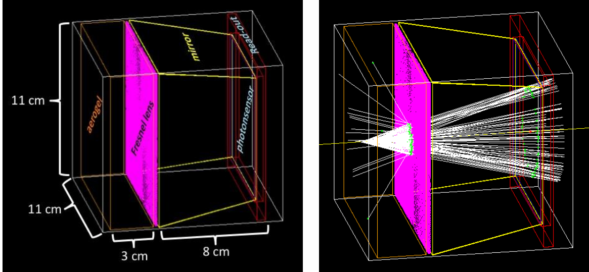
Figure 2.2.1.3. Figure on the left shows the modular RICH detector design in GEMC simulation framework. White wireframe is the detector holder box. Orange wireframe is a 3-cm thick aerogel with refractive index 1.05. In magenta is the Fresnel lens with 100 grooves, focusing the Cherenkov radiation. Four mirrors (yellow) are placed at the top, bottom, left, and right of the detector. At the back (in red) of the detector are photosensors and readout electronics. Figure on the right shows a single negatively-charged pion passing through the detector. The pion emits Cherenkov photons inside the aerogel. Those photons are focused by a Fresnel lens before arriving at the photosensors.
