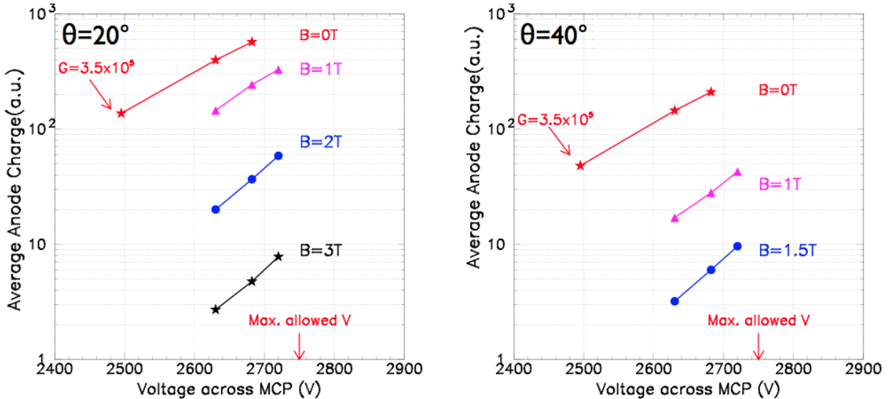
Figure 4.1.3. Average anode charge per pulse as a function of V_{MCP-MCP} for several values of the magnetic field B and two angles \theta between the MCP-PMT and the B-field axes, 20^\circ and 40^\circ . By increasing V_{MCP-MCP} to 99% of the maximum allowed value, the gain of 3.5 \times 10^5 at 0 T was recoverable to < 2 T at \theta = 20^\circ and to < 1 T at \theta = 40^\circ .
