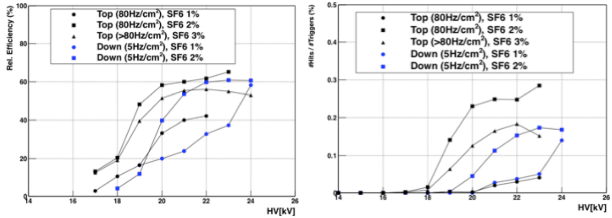
Figure 1.2.1.3. The left plot shows efficiency vs. high voltage results for different locations and gas mixtures. The right plot shows the hit ratios over the number of triggers.
