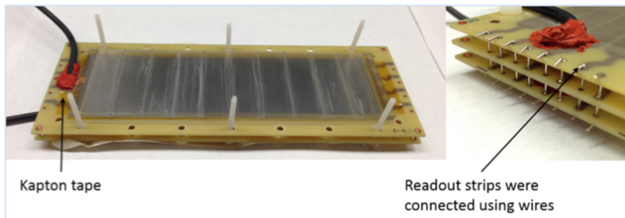
Figure 1.2.2.1. A photograph showing the inner structure of the 3D printed gas gap.
