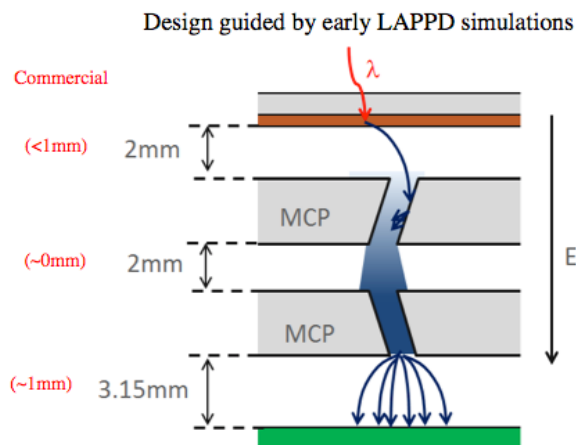
Figure 4.2.13. Basic setup of the LAPPD stack. Note that the gap distances are significantly larger than those in a typical commercial device (shown in red type at the left side). This will create opportunity for a transverse field to upset the gain amplification process in the LAPPD stack.
