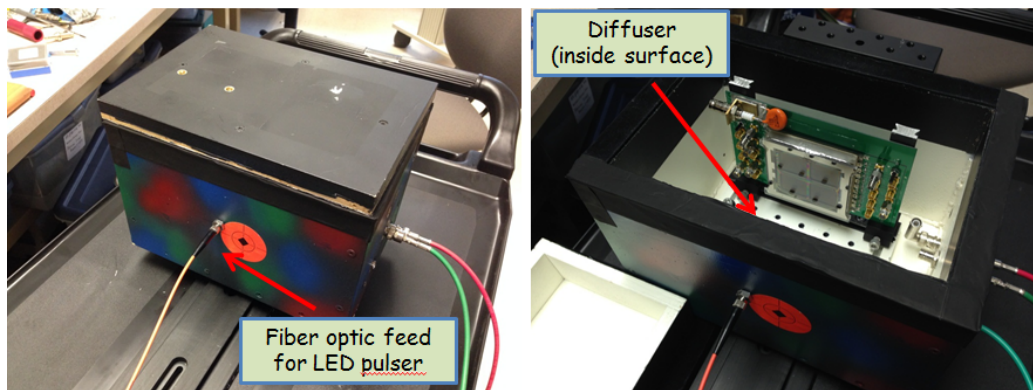
Figure 4.2.1. Photograph of small dark box setup for testing LAPPD sample in a high B field. The light source is a 370 nm pulsed LED connected via a 5 meter fiber optic to the dark box. A diffuser on the inside surface (not seen in photo) spreads the light from the fiber optic in a uniform illumination of the LAPPD faceplate. The box can be mounted on an optical rail to allow controlled insertion into a magnetic field.
