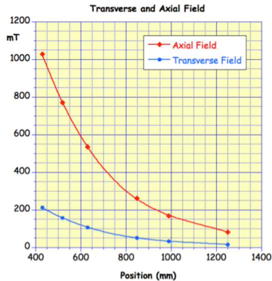
Figure 4.2.8. Magnitudes of the actual axial and transverse components of the B field as function of the position of the sample relative to the entrance face of the magnet bore.
