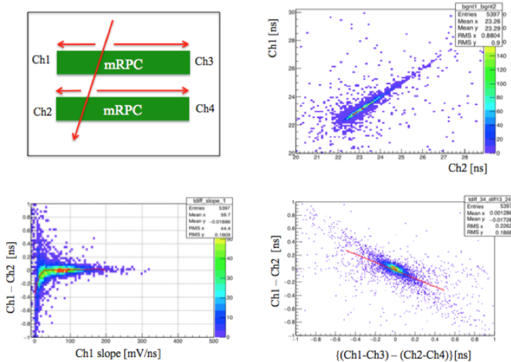
Figure 1.2.1.4. The top left diagram shows the channel mapping for the readout from the two mRPCs. The top right shows the time correlation between the channel 1 and 2. The bottom left plot shows the correlation between the time difference and the rise-time of channel 1. The bottom right plot shows the correlation between the time difference and hit position difference calculated from the signal propagation of all channels.
