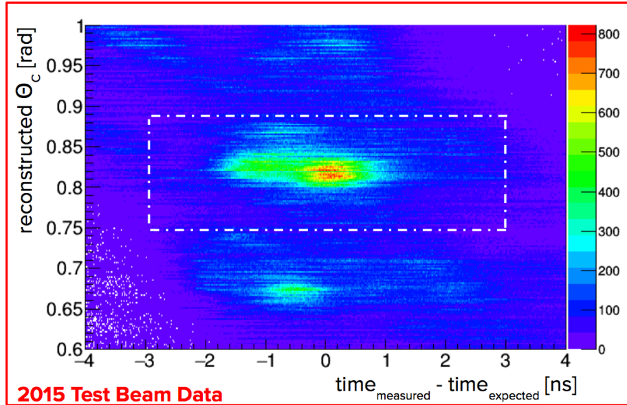
Figure 3.12. Cut on reconstructed single-photon Cherenkov angle as a function of time (measured - expected) for 2015 CERN beam data. 7 GeV/c beam is entering the setup at 90° angle (setup with air-gap lens).
