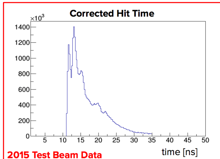
Figure 3.5. Corrected hit time of an example pixel.
