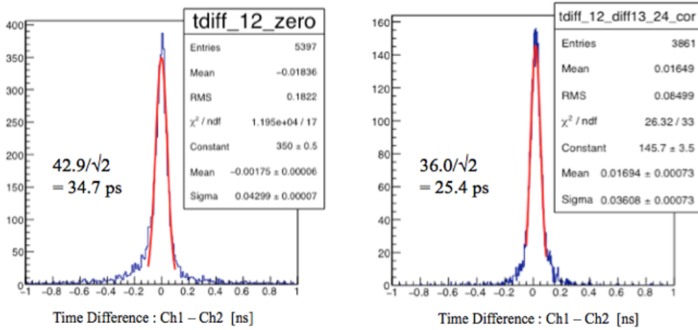
Fig 1.2.1.5. The left plot shows the time difference distribution with a Gaussian fitting before the corrections. The right plot shows the time difference distribution with a Gaussian fitting after the corrections.
