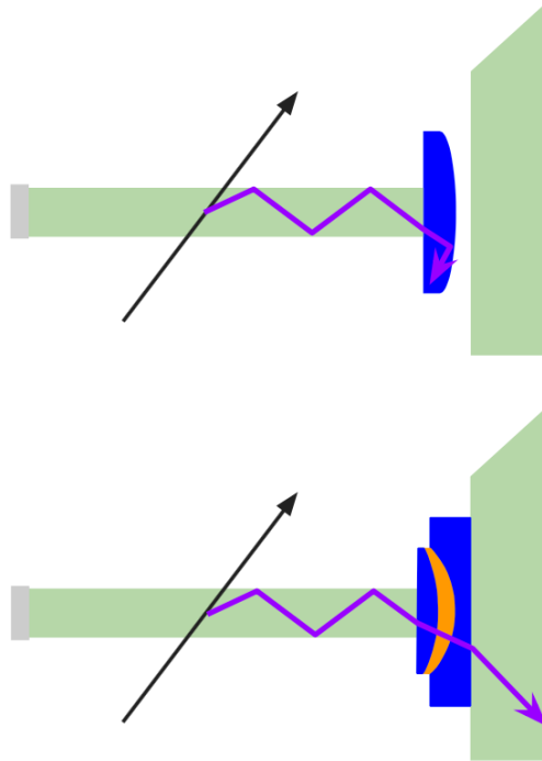
Figure 3.6. Schematic diagram of photon propagation from the bar to the prism for the configuration with an air-gap lens (top) and the three-component lens (bottom) .
