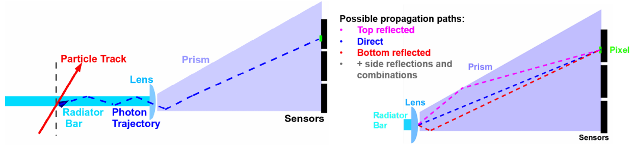
Figure 3.8. Schematic diagram of the reconstruction concept, with one example photon track emitted from a particle. The direction vector k is an estimator of the origin vector k_{\text{org}} , and is used to reconstruct \theta_c . On the right, three examples for possible propagation paths of the photon from the center of the bar end to one of the pixels are shown.
