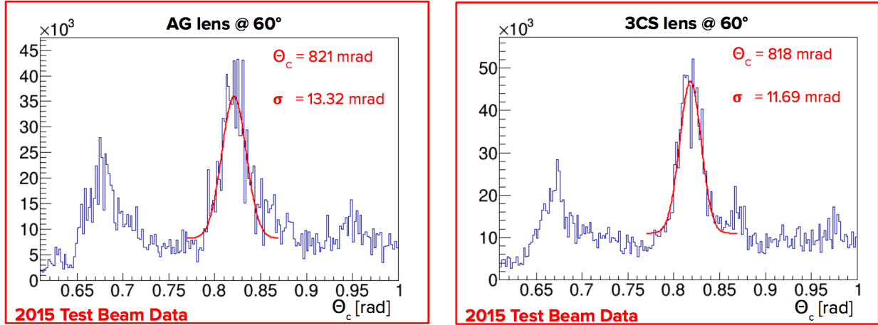
Figure 3.10. Reconstructed single-photon Cherenkov angle from the 2015 CERN beam data for a 7 GeV/c momentum and 60° polar angle. Left: Setup with air-gap lens. Right: Setup with 3-component lens.
