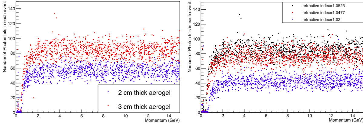
Figure 2.2.1.5. Number of Cherenkov Photon Hits detected by the Photon Sensor vs. momentum (in range 0 to 15 GeV) of incident pions. Left: fixed refractive index (1.0523), but with different thicknesses (3 cm in red, and 2 cm in blue) of the aerogel. Right: simulation with fixed aerogel thickness (3 cm) but with different refractive index (1.0523 in black, 1.0477 in red, and 1.02 in blue).
