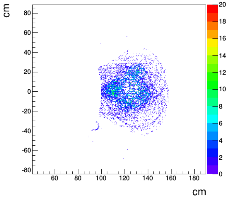
Figure 2.2.2.7: The spatial distribution of the photon hits on the detector plane.
