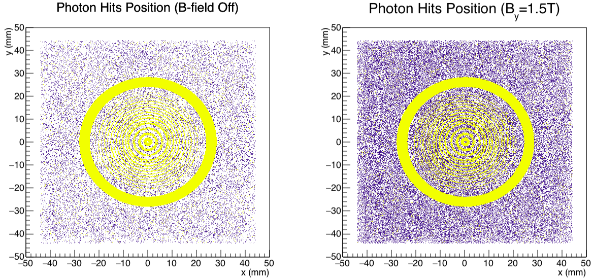
Figure 2.2.1.10. Photon hits on the photosensor with mother particle id which is shown in color. Cherenkov photons which are emitted by 100,000 incident particles, muon (yellow) with 9 GeV, form rings on the photosensor. Cherenkov photons emitted by delta ray electrons are indicated in purple. Plot on the left is from simulation without magnetic field. Plot of the right is from simulation with uniform 1.5-T y-direction magnetic field.
