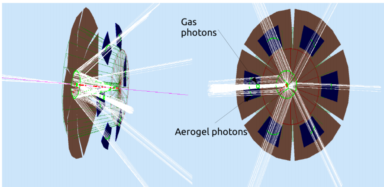
Figure 2.2.2.7. Full angle view of the mirror based RICH detector, with a pion event of momentum 30 GeV/c.
