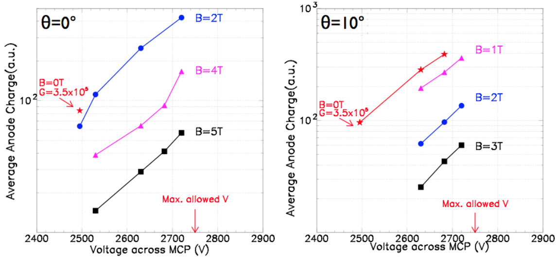
Figure 4.1.2. Average anode charge per pulse as a function of V_{MCP-MCP} for several values of the magnetic field B and two angles \theta between the MCP-PMT and the B-field axes, 0^\circ and 10^\circ . The average anode charge is proportional to the gain of the sensor and is our control quantity for gain evaluation. As V_{MCP-MCP} increases, the gain increases exponentially, which allows the gain of 3.5 \times 10^5 at 0 T to be recoverable up to 5 T at \theta = 0^\circ and up to 3 T at \theta = 10^\circ .
