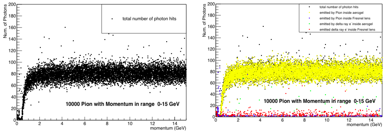
Figure 2.2.1.7. Number of Photons detected on Photosensor in Each Event vs. Momentum of Incident Pions. Black dots on both plots represent the sum of the numbers of signal, and background Cherenkov photons detected. Plot on the right shows the number of signal Cherenkov photons (Yellow), and background Cherenkov photons from different sources, counted in each event. Blue, green, and red dots represent background Cherenkov photons emitted by incident Pions inside Fresnel lens, by delta ray electrons inside aerogel, and by delta ray electrons inside Fresnel lens, respectively.
