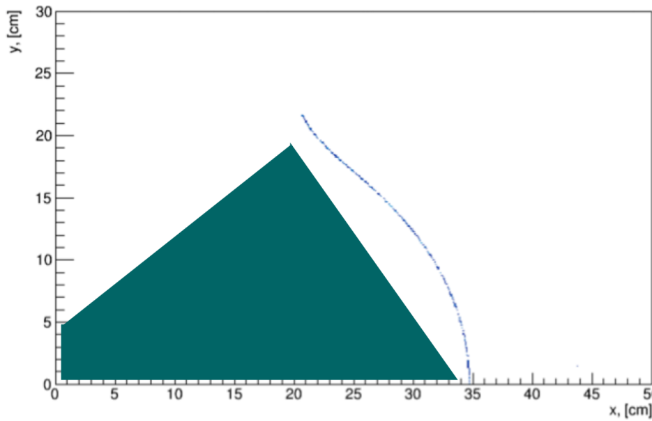
Figure 3.20. Geant4 simulation of the 3-layer lens with a tilted focal plane.
