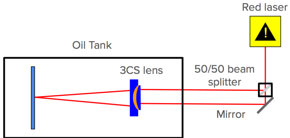
Figure 3.17. Schematic diagram of the optical setup to map the focal plane of the high-refractive lens as a function of rotation angle of the lens.
