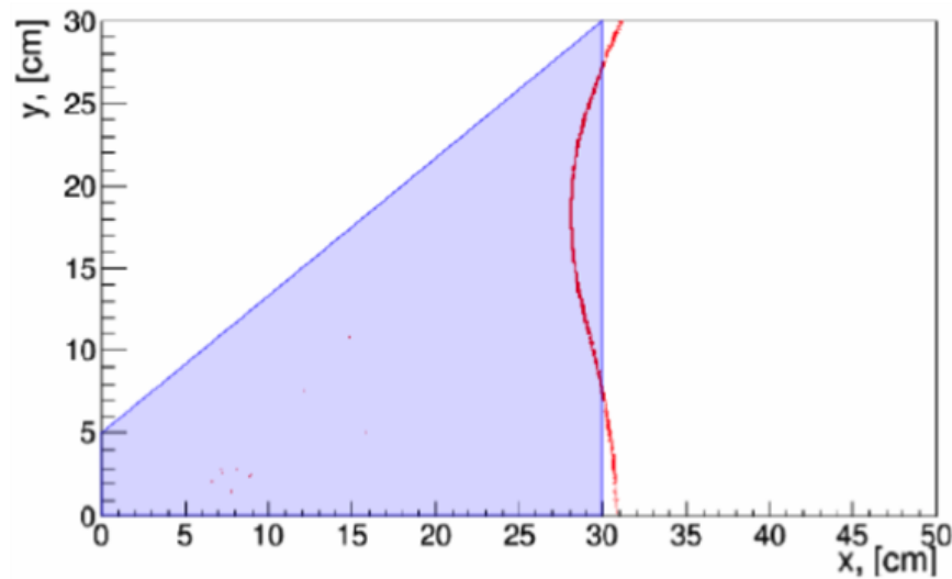
Figure 3.16. Simulated focal plane for the three-layer lens in Geant4.
