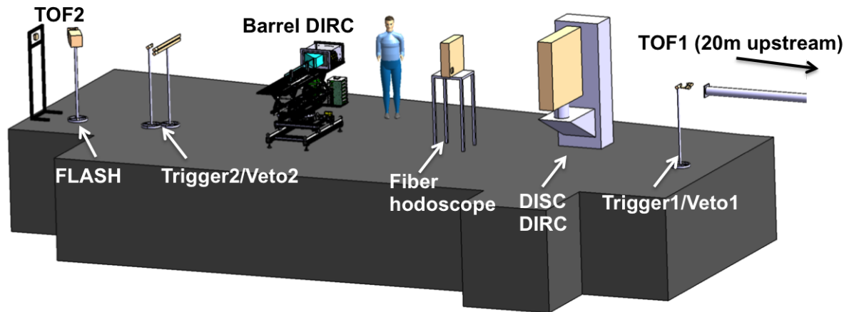
Figure 3.4. Arrangement of the prototype elements used in the 2015 test beam at CERN.
