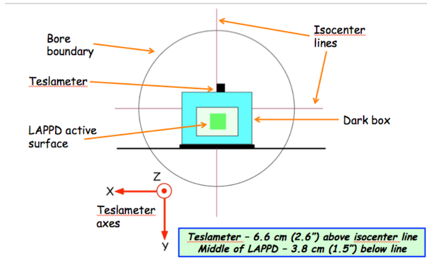
Figure 4.2.5. Schematic showing the position of the LAPPD relative to the symmetry axis of the MRI magnet.
