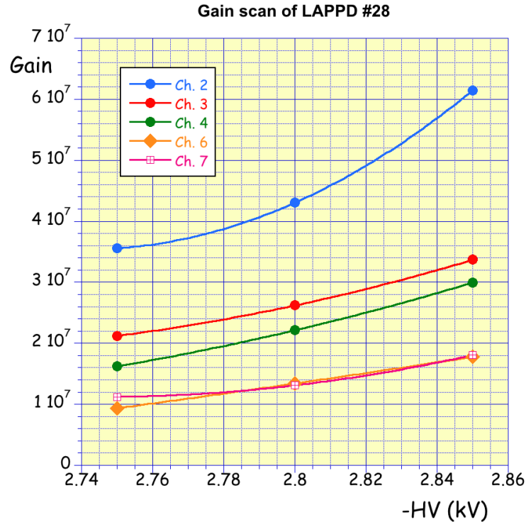
Figure 4.2.2. Gain scan of the live channels of the LAPPD using SPE spectra to determine the gain. Channels 1,5, and 9 are not shown as the glass frame within the LAPPD structure blocks the amplification process. Channel 8 had a very weak signal. Channels 3 and 6 were chosen for the magnetic field test – one from the upper half and the other from the lower half of the LAPPD. The HV was fixed at -2.8 kV during the test.
