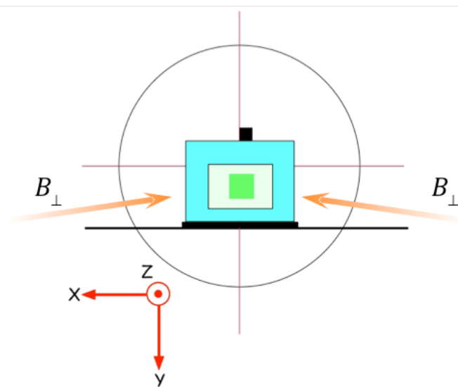
Figure 4.2.6. As on Fig. 4.2.5, but here we show the orientations of the transverse field vectors.
