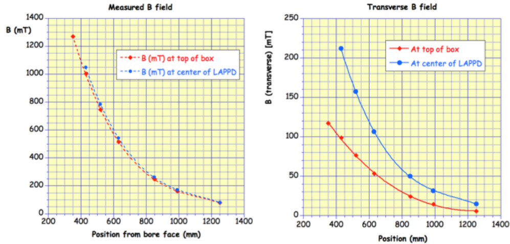
Figure 4.2.7. The B-field data collected shows that the transverse field differs significantly between the teslameter position during the tests and the actual values at the center of the LAPPD faceplate (RH plot). In contrast, the total B field magnitude differs only slightly (LH plot).
