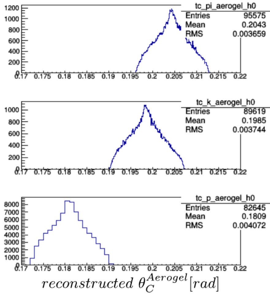
Figure 2.2.2.8: Distributions for the reconstructed aerogel cherenkov angles (sample of 1000 traks with momentum 10 GeV/c at polar angle of 25°) for \pi , K, p (from top to bottom).
