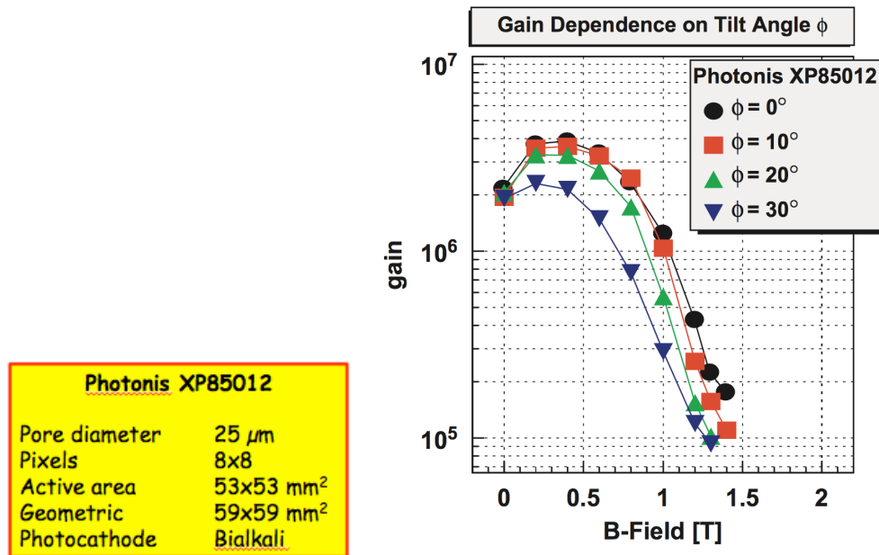
Figure 4.2.12. From reference [3], a plot showing the gain changes in the Photonis XP85012, a commercial MCP-PMT, which is comparable to the LAPPD. The results show that the commercial device has far greater tolerance to a high magnetic field compared to the current LAPPD sample. Examination of the structure of the prototype LAPPD reveals why this follows.
