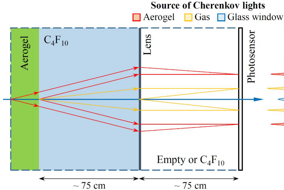
Figure 2.2.2.4: Options for a dual-radiator RICH detector for the EIC: a concept using a lens for focusing.
