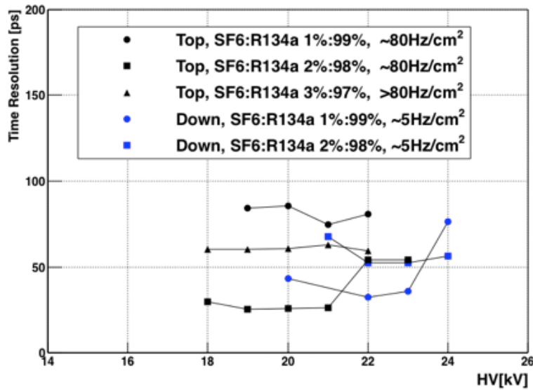
Figure 1.2.1.6. Time resolution results from the different flux rates and gas mixtures as a function of the applied high voltage.
