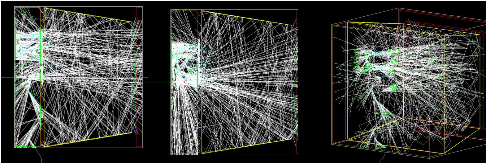
Figure 2.2.1.9. GEMC event display shows Delta Ray electrons (cyan) generated by single incident muon (green) move in spiral trajectory inside the aerogel due to the presence of magnetic field. Photons are shown in white. From left to right: side view, bird view, and front view of modular RICH detector.
