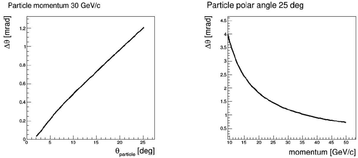
Figure 2.2.2.11: (left panel) induced error by the magnetic field on the Cherenkov angle measurement ( \sigma_B = \Delta\theta/\sqrt{2} per single p.e.) as a function of the polar angle of a charged pion of momentum 30 GeV/c (in the RICH region). (right panel) \Delta\theta as a function of the track momentum at a fixed value of the polar angle, 25^\circ .
