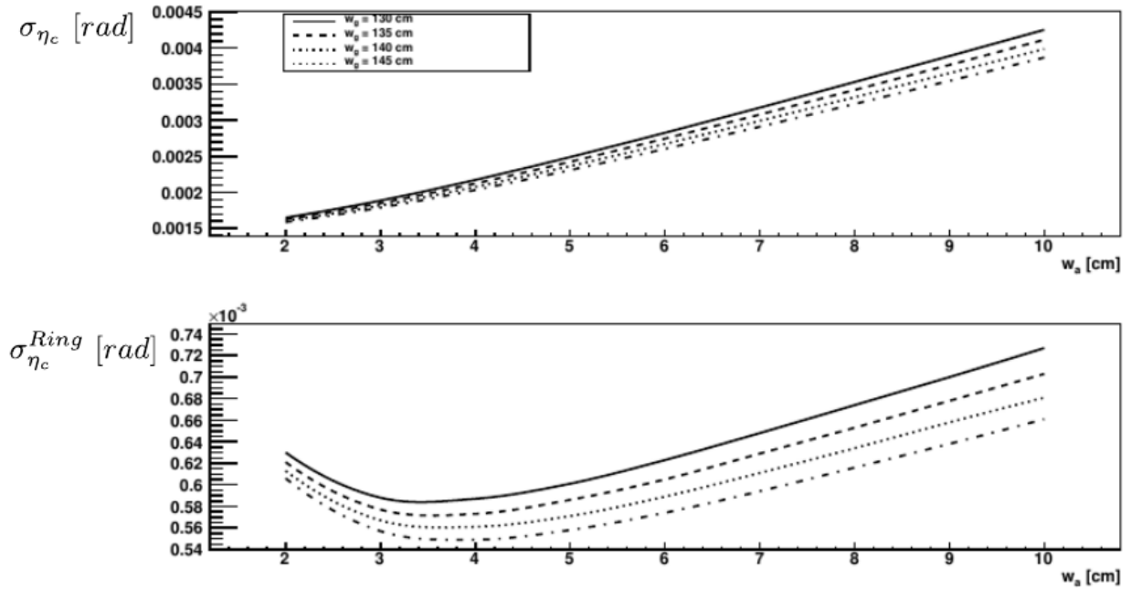
Figure 2.2.2.2. (Upper panel) The sigma on the Cherenkov angle (for n = 1.02 , the maximum cherenkov angle is 0.198 rad) is plotted as a function of thickness of the Aerogel radiator ( w_a ) for different thickness of the gas box ( w_g ); (lower panel) is the resolution on the ring (the upper plot divided by the square root of the number of emitted photoelectrons) plotted as a function of the aerogel thickness. Both for a pion at \langle p \rangle = 5 GeV/c.
