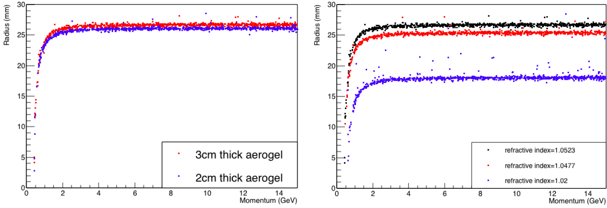
Figure 2.2.1.4. Plots of Cherenkov ring radius versus momentum (in range 0 to 15 GeV) for incident pions. Left: simulations with fixed refractive index n=1.0523 of aerogel, but with different aerogel thicknesses (3 cm in red, and 2 cm in blue). Right: simulation with fixed aerogel thickness (3 cm) but with different refractive index (1.0523 in black, 1.0477 in red, and 1.02 in blue).
