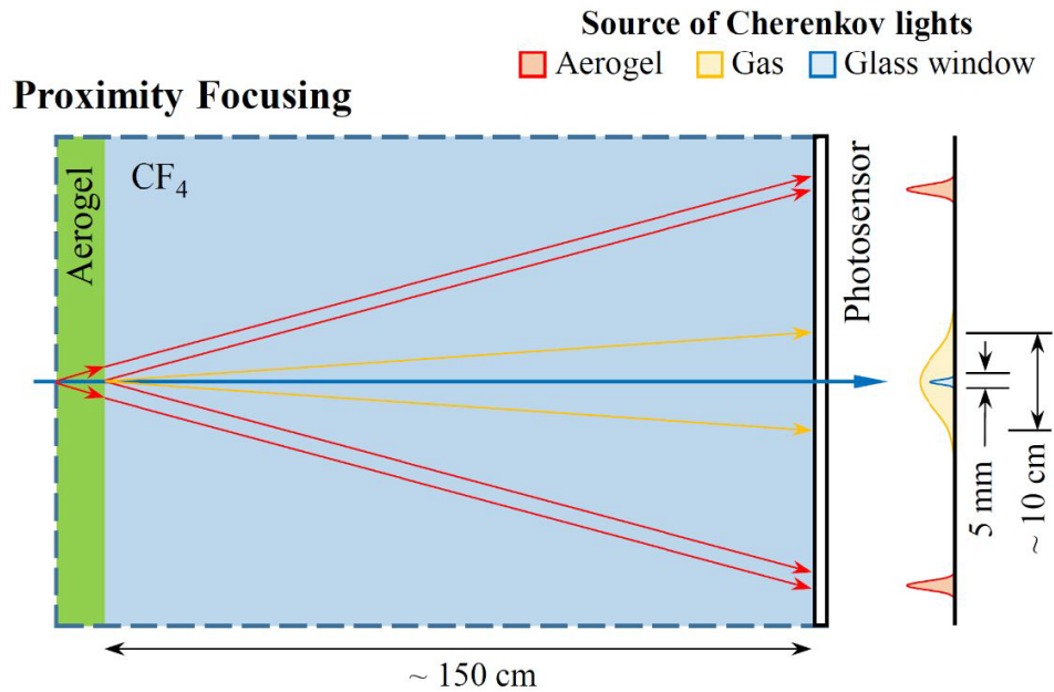
Figure 2.2.2.1: Options for a dual-radiator RICH detector for the EIC: a concept using proximity focusing.
