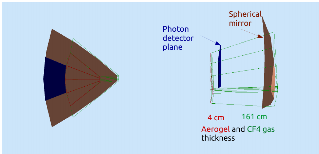
Figure 2.2.2.6. A frontal (left) and lateral (right) views of a sector of the mirror based RICH are shown.
