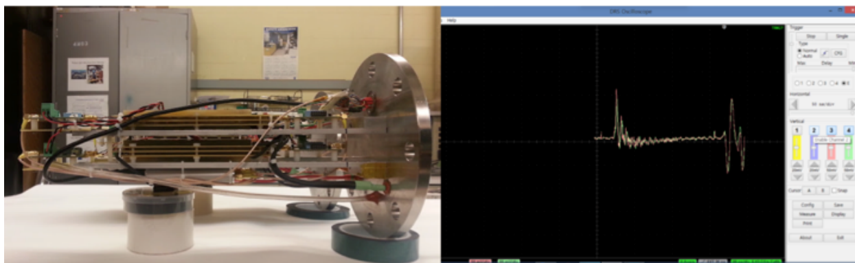
Figure 1.2.2.2. The left picture shows the two 3D printed gas gap mRPCs stacked on the rail of the gas fringe. The right screen shot shows signals (first peak from left to right) captured at the waveform analyzer.
