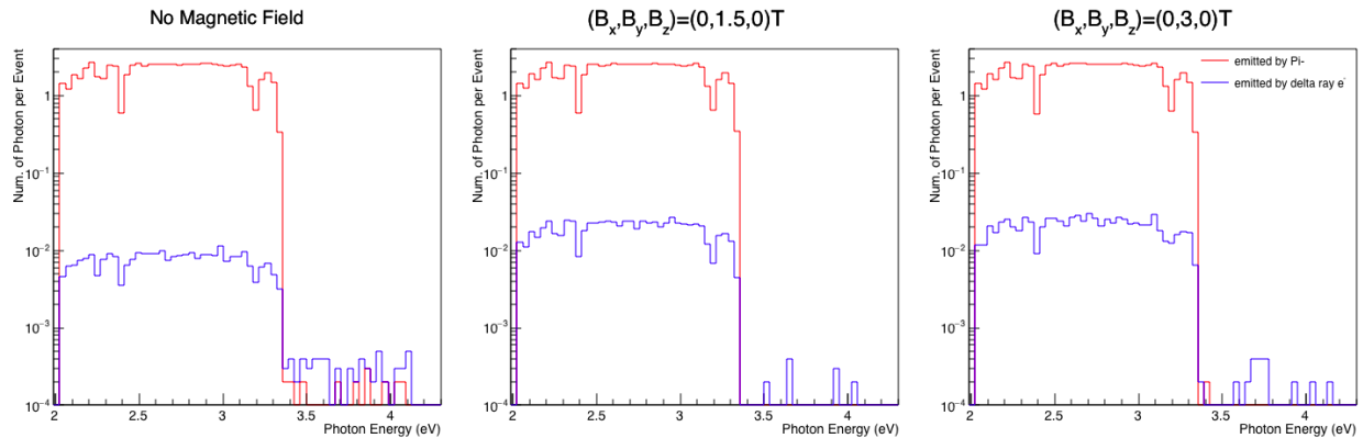
Figure 2.2.1.11. Photon energy distribution normalized to the total number of events. Red line represents the photons emitted by incident particles which are negatively-charged pions. Blue lines represent the background photons emitted by delta ray electrons. Plots from left to right are from simulations without magnetic field, with uniform 1.5-T y-direction magnetic field, and with uniform 3-T y-direction magnetic field, respectively.
