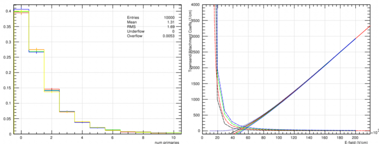
Figure 1.2.3.1. The left picture shows the number of primary electrons per 105 um gas gap, for SF 6 percentages of 1, 2, 3, and 4% and an E-field of 152K V/cm. The right figure shows the Townsend and Attachment coefficients as a function of E-field (solid and dashed lines, respectively).
