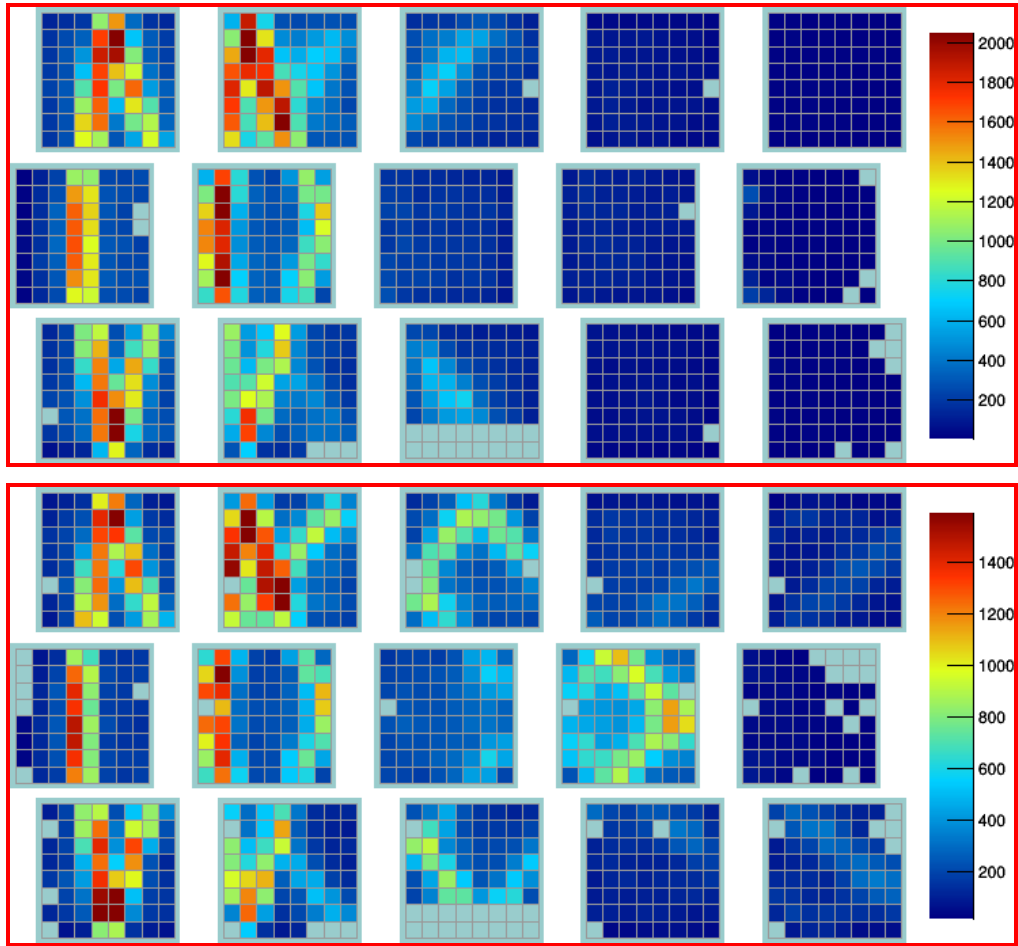
Figure 3.7. Distribution of the number of hits per MCP-PMT pixel in the 2015 test beam data for a configuration using an air-gap lens (top) and a 3-layer lens (bottom).
