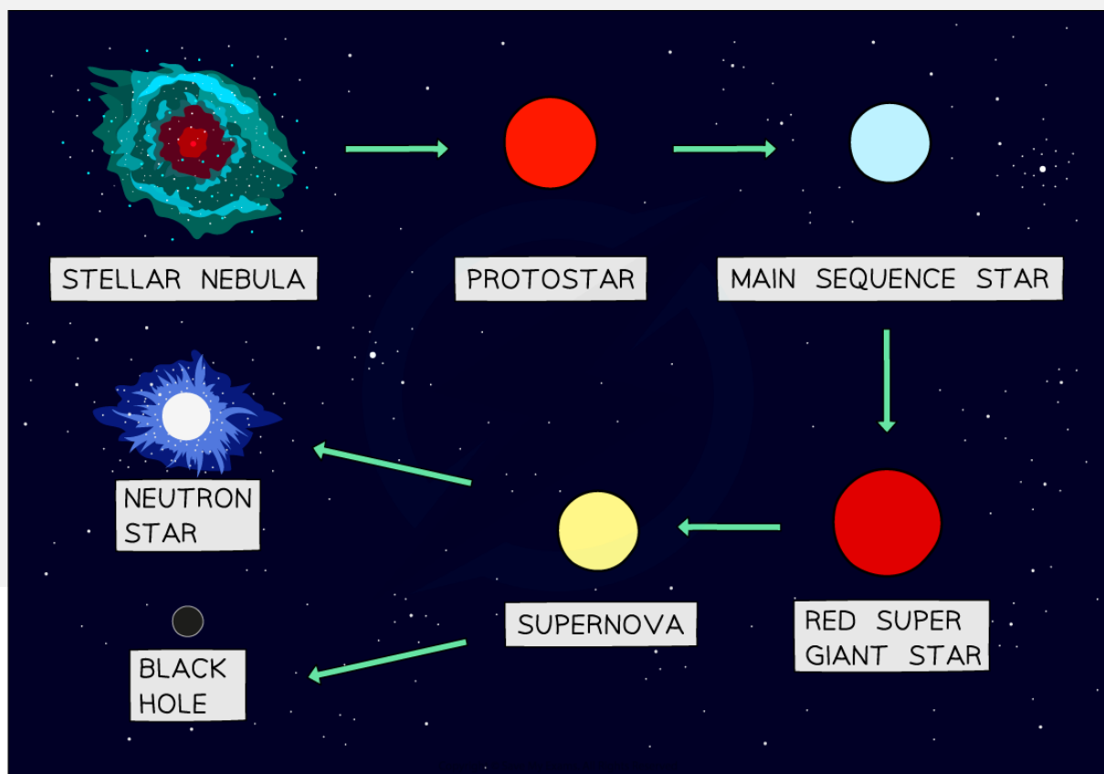
The life cycle of a star much larger than our Sun
