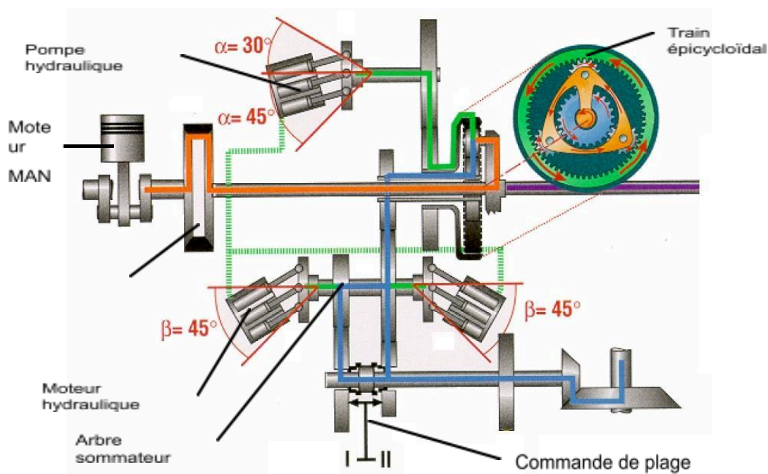
Figure 13: Transmission Fendt 900 Vario
