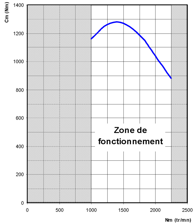
Figure 8 : Courbe C_m = f(N_m)
