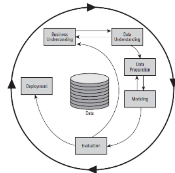
Gambar 1. CRISP-DM
