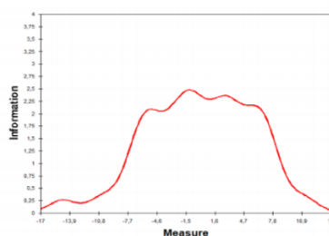
Figure 1. Test Information Function
