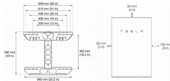
Figure 19: Powerwall 2 Mounting Bracket Dimensions and Space Requirements
