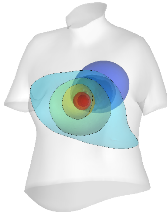
Figure 1. Extracellular potential distribution in the torso volume.
