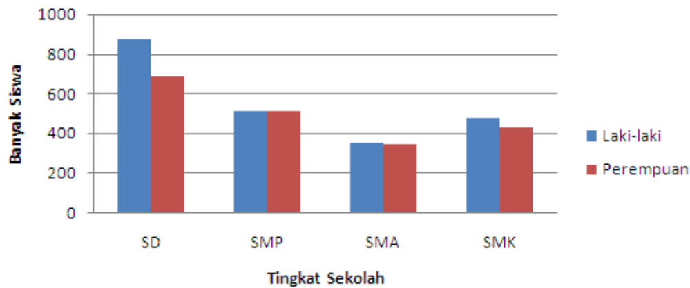
Gambar 1. Contoh Diagram
