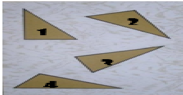
Gambar 1. Four congruent right triangles attached to a sheet of paper in different positions.
