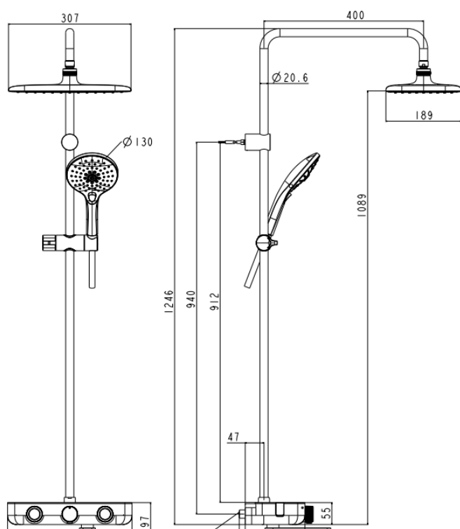
DIMENSIONAL DRAWING
