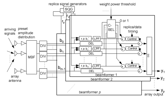
Figure 1. Proposed beam former
