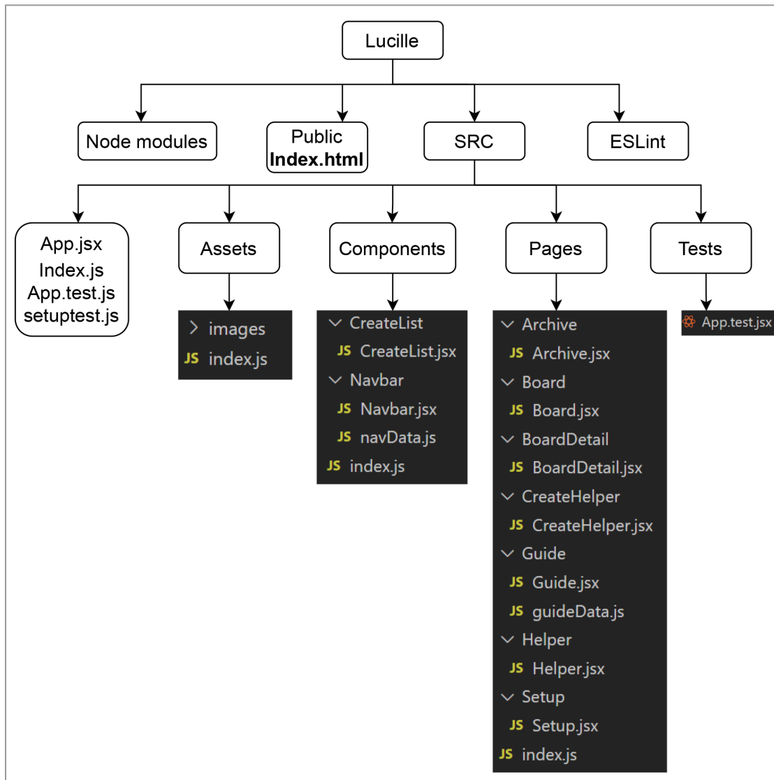
Figure 18 : File structure of Lucille application
