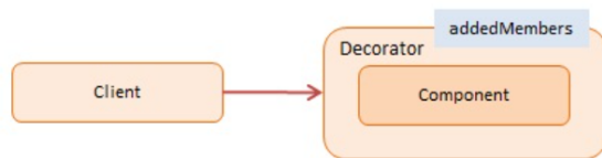
Figure 11: UML diagram Decorator design pattern in javascript ( JavaScript Decorator Design Pattern - Dofactory, 2022 )
