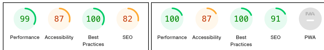
Figure 16: Performance measurement before and after converting assets to .svg format.
