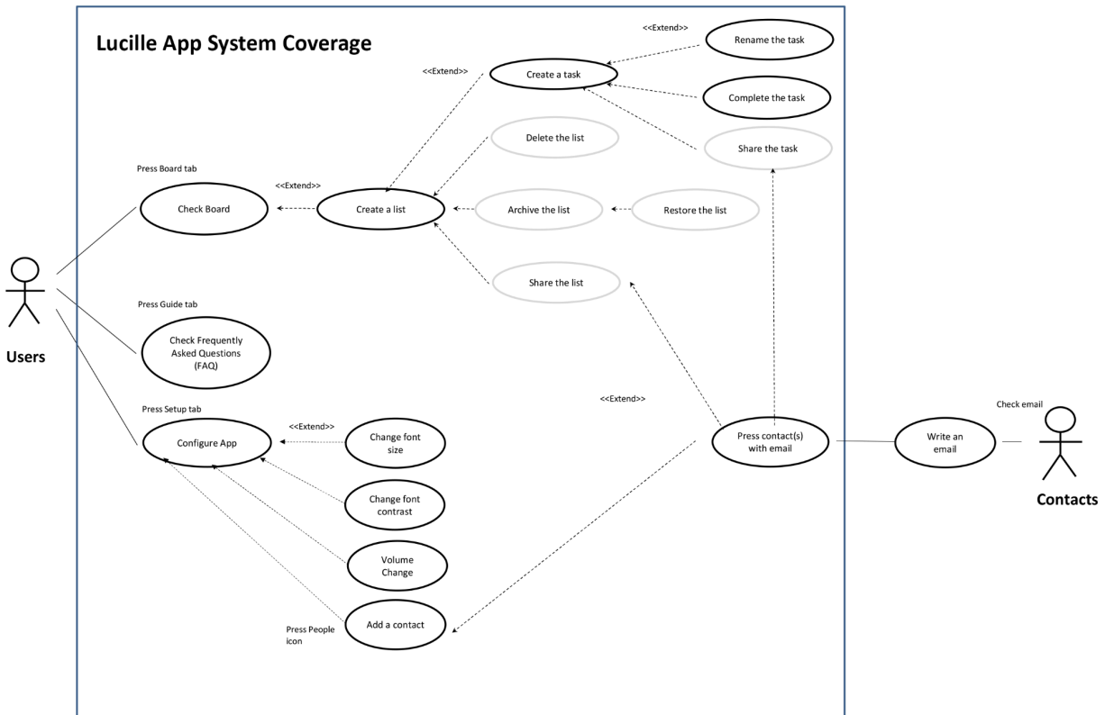
Figure 10: UML diagram
