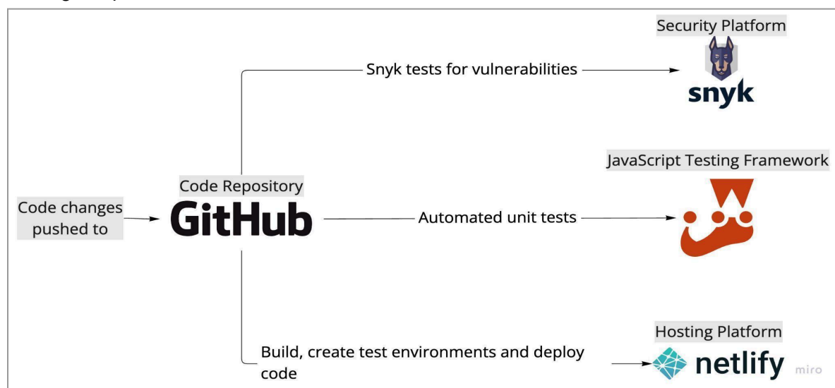
Figure 14: Production, staging and deployment.
